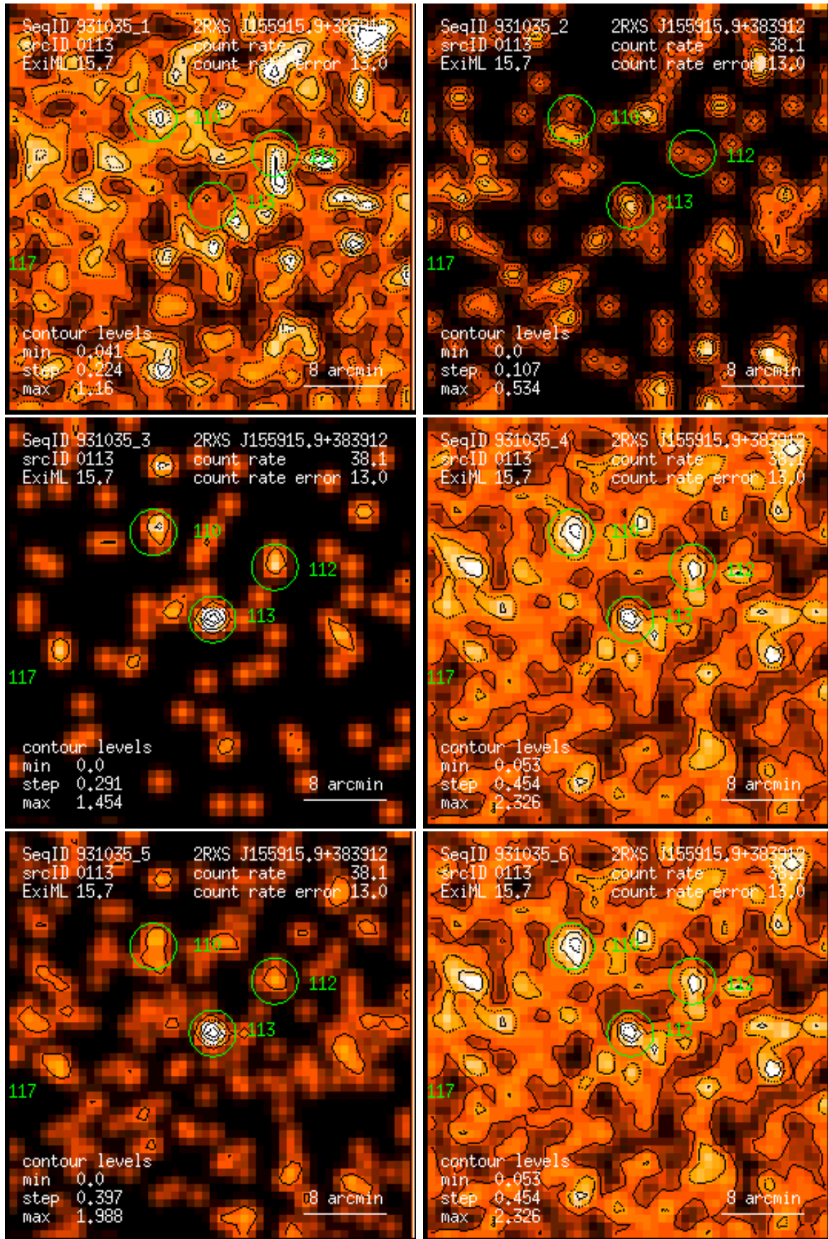
Figure 113: RASS 931035: detection 0113: band rate images, Gaussian filter: (1) PSPC channels 11 – 41, (2) 52 – 90, (3) 91 – 201, (4) 11 – 235, (5) 52 – 201, (6) 11 – 201. Broad band rates in counts/ks. Band rate contour levels in counts/ks/arcmin 2 .
