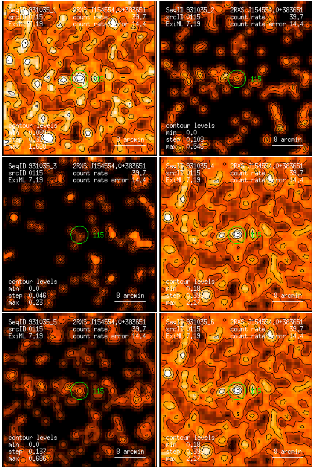
Figure 115: RASS 931035: detection 0115: band rate images, Gaussian filter: (1) PSPC channels 11 – 41, (2) 52 – 90, (3) 91 – 201, (4) 11 – 235, (5) 52 – 201, (6) 11 – 201. Broad band rates in counts/ks. Band rate contour levels in counts/ks/arcmin 2 .
