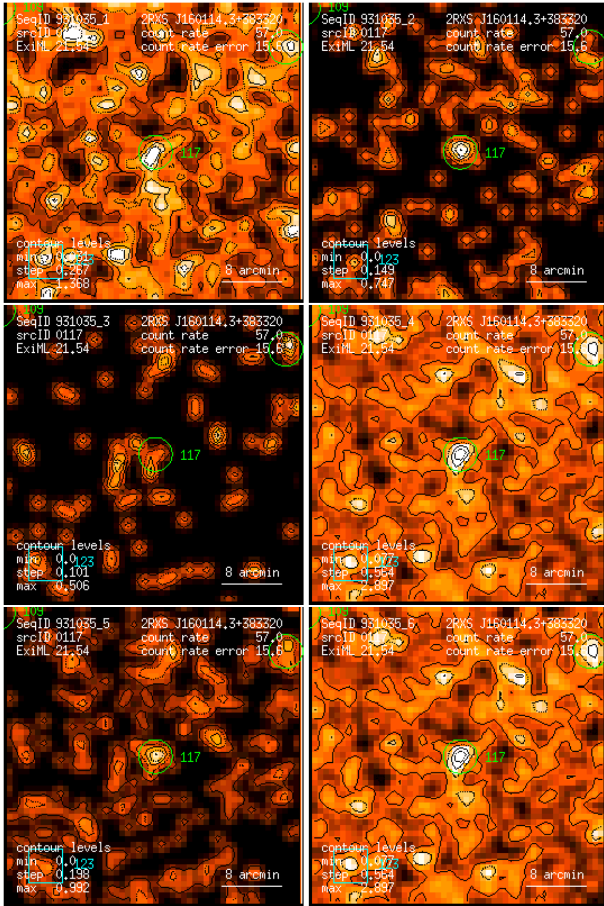
Figure 117: RASS 931035: detection 0117: band rate images, Gaussian filter: (1) PSPC channels 11 – 41, (2) 52 – 90, (3) 91 – 201, (4) 11 – 235, (5) 52 – 201, (6) 11 – 201. Broad band rates in counts/ks. Band rate contour levels in counts/ks/arcmin 2 .
