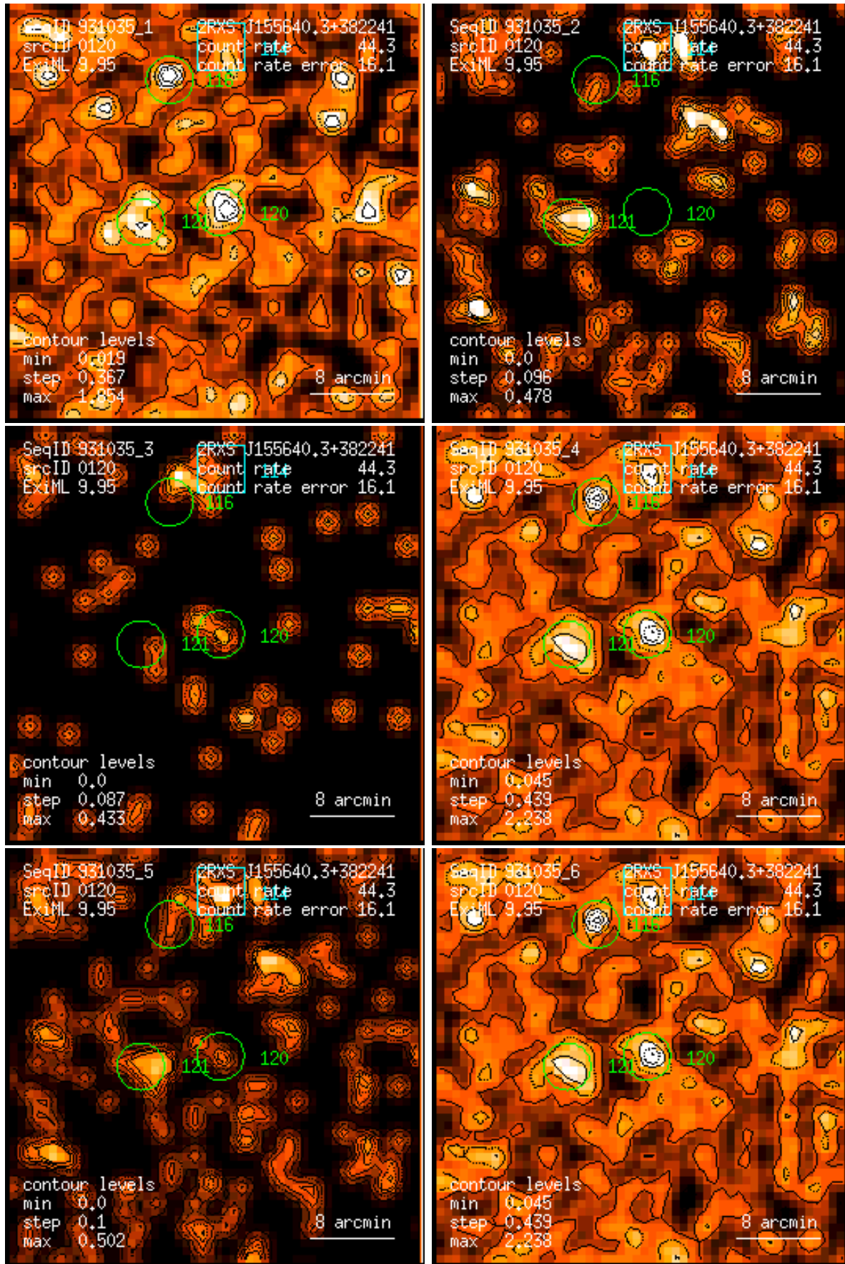
Figure 120: RASS 931035: detection 0120: band rate images, Gaussian filter: (1) PSPC channels 11 – 41, (2) 52 – 90, (3) 91 – 201, (4) 11 – 235, (5) 52 – 201, (6) 11 – 201. Broad band rates in counts/ks. Band rate contour levels in counts/ks/arcmin 2 .
