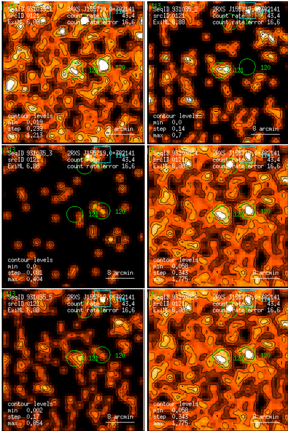
Figure 121: RASS 931035: detection 0121: band rate images, Gaussian filter: (1) PSPC channels 11 – 41, (2) 52 – 90, (3) 91 – 201, (4) 11 – 235, (5) 52 – 201, (6) 11 – 201. Broad band rates in counts/ks. Band rate contour levels in counts/ks/arcmin 2 .
