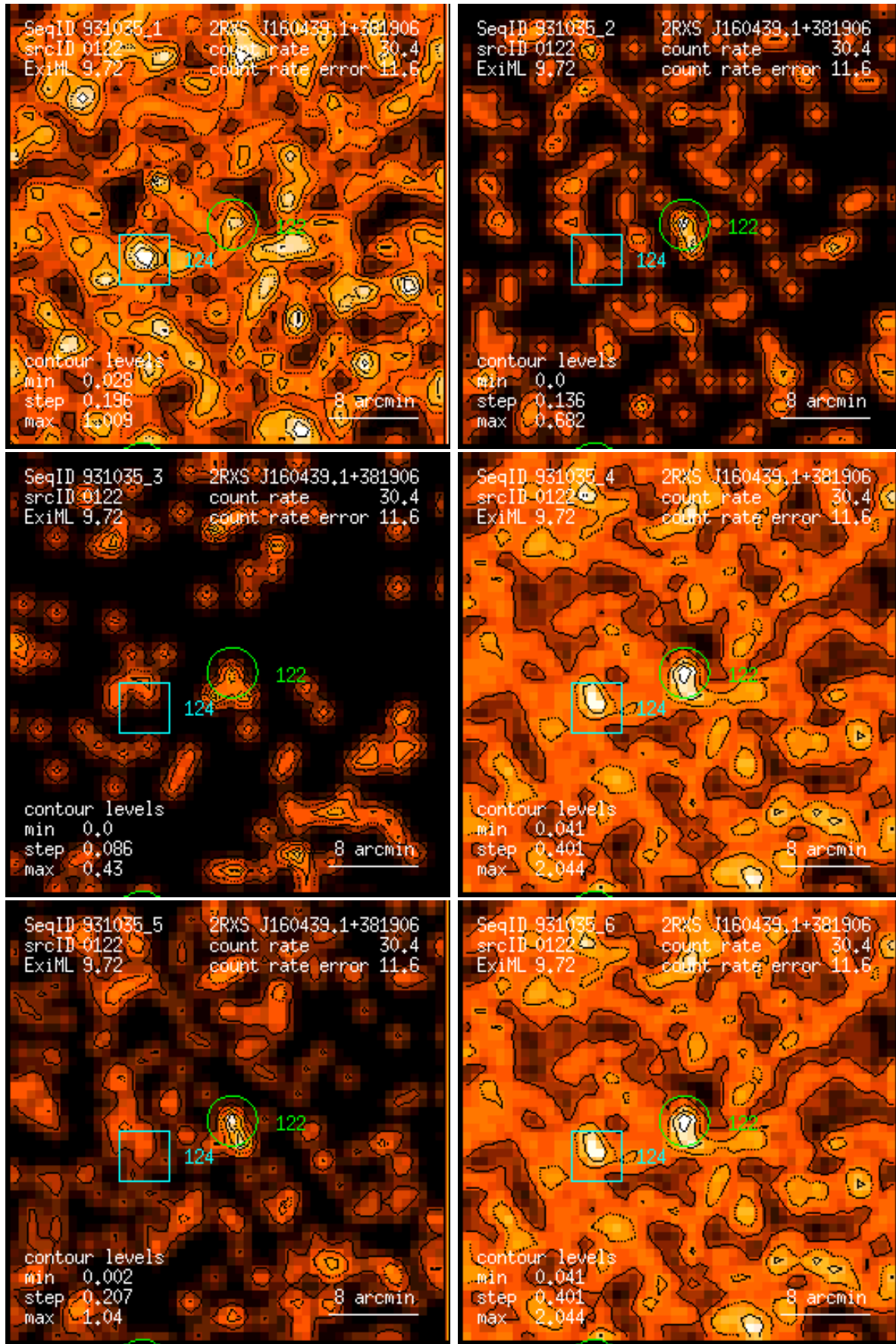
Figure 122: RASS 931035: detection 0122: band rate images, Gaussian filter: (1) PSPC channels 11 – 41, (2) 52 – 90, (3) 91 – 201, (4) 11 – 235, (5) 52 – 201, (6) 11 – 201. Broad band rates in counts/ks. Band rate contour levels in counts/ks/arcmin 2 .
