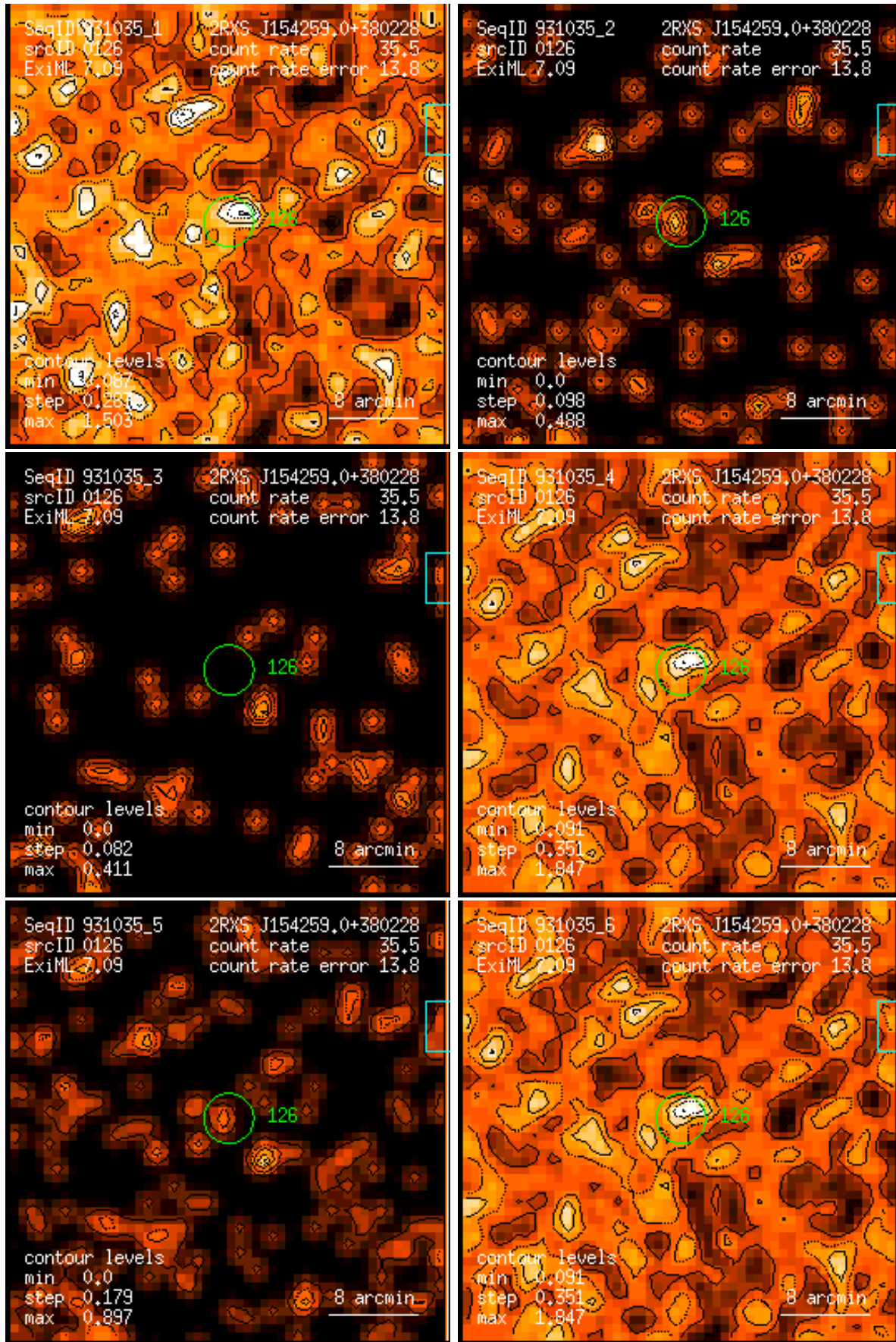
Figure 126: RASS 931035: detection 0126: band rate images, Gaussian filter: (1) PSPC channels 11 – 41, (2) 52 – 90, (3) 91 – 201, (4) 11 – 235, (5) 52 – 201, (6) 11 – 201. Broad band rates in counts/ks. Band rate contour levels in counts/ks/arcmin 2 .
