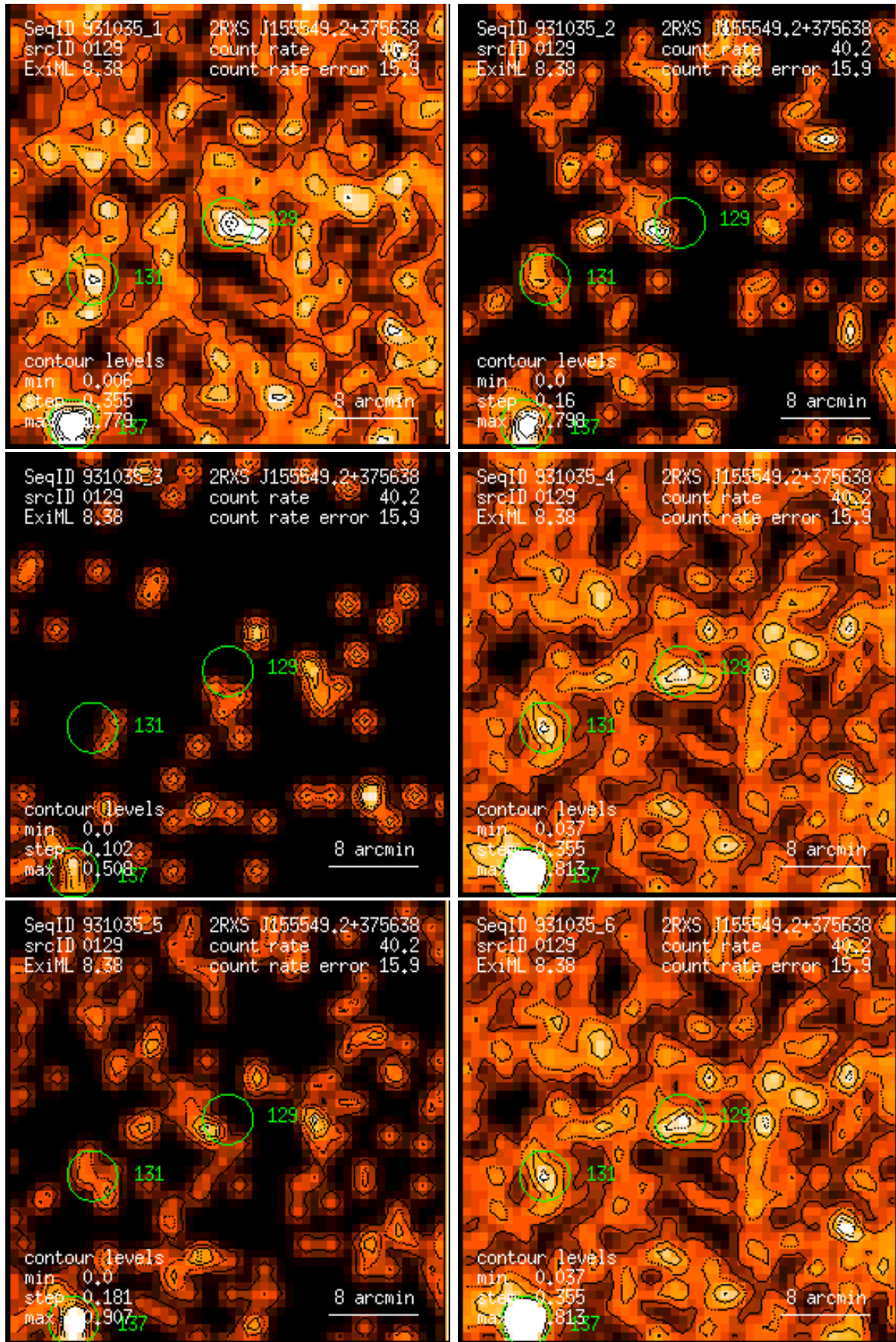
Figure 129: RASS 931035: detection 0129: band rate images, Gaussian filter: (1) PSPC channels 11 – 41, (2) 52 – 90, (3) 91 – 201, (4) 11 – 235, (5) 52 – 201, (6) 11 – 201. Broad band rates in counts/ks. Band rate contour levels in counts/ks/arcmin 2 .
