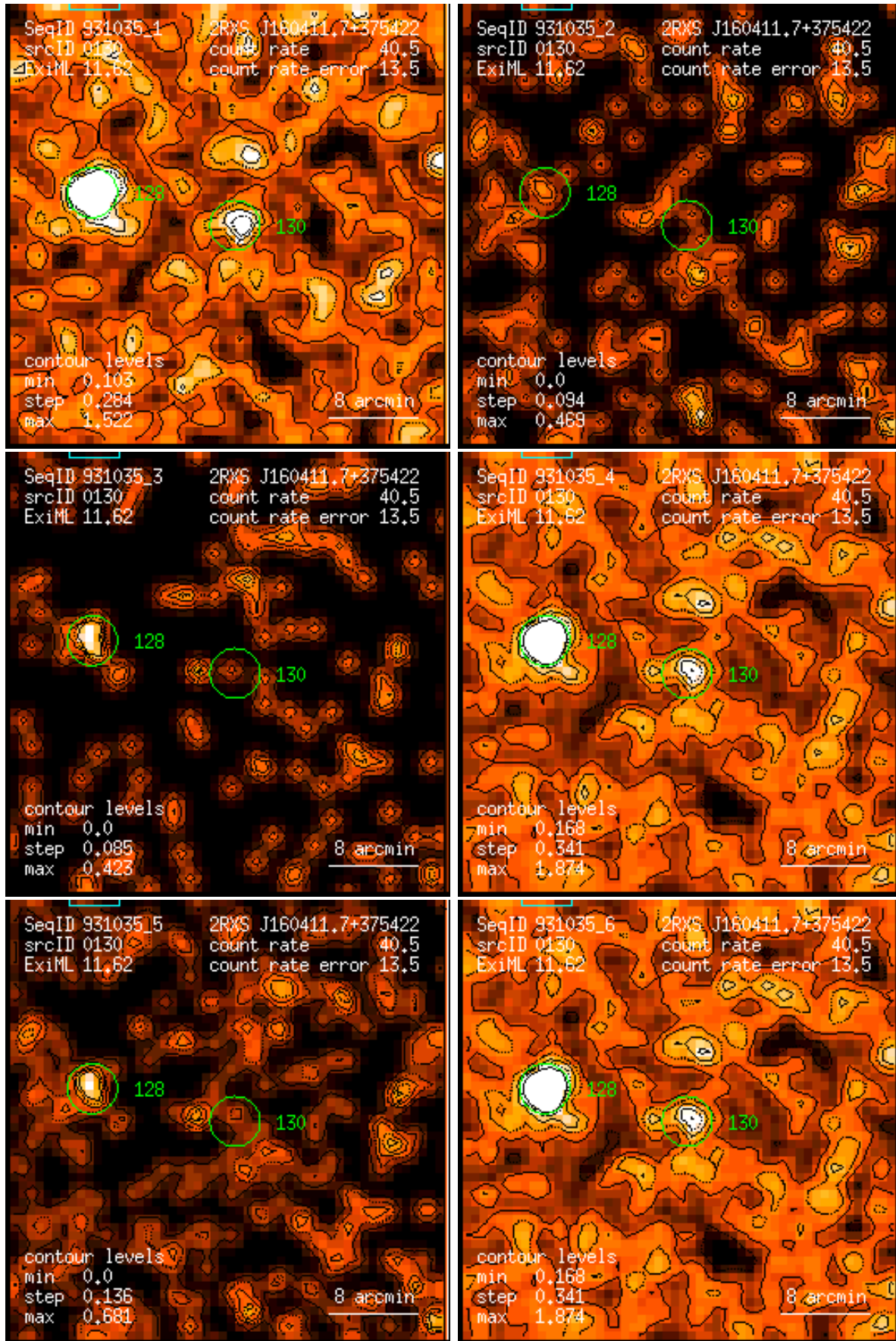
Figure 130: RASS 931035: detection 0130: band rate images, Gaussian filter: (1) PSPC channels 11 – 41, (2) 52 – 90, (3) 91 – 201, (4) 11 – 235, (5) 52 – 201, (6) 11 – 201. Broad band rates in counts/ks. Band rate contour levels in counts/ks/arcmin 2 .
