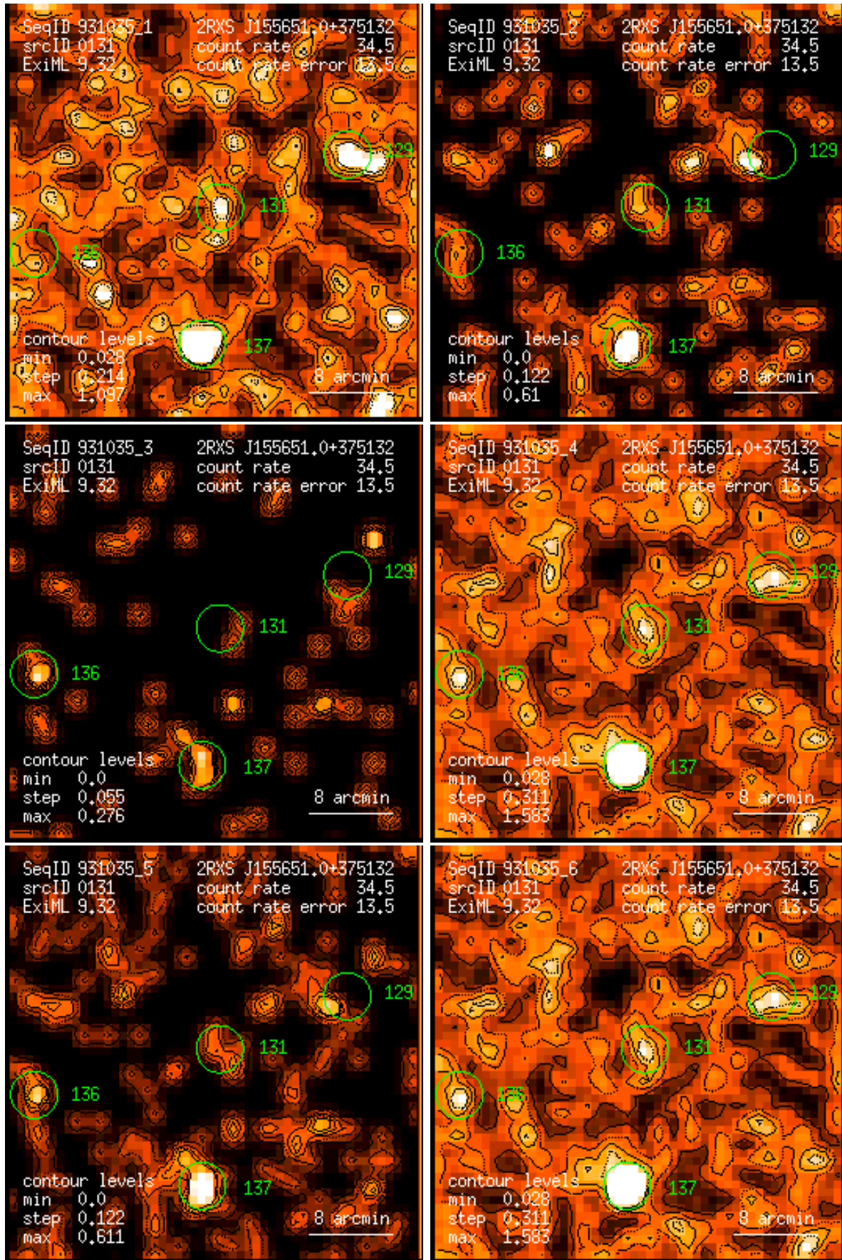
Figure 131: RASS 931035: detection 0131: band rate images, Gaussian filter: (1) PSPC channels 11 – 41, (2) 52 – 90, (3) 91 – 201, (4) 11 – 235, (5) 52 – 201, (6) 11 – 201. Broad band rates in counts/ks. Band rate contour levels in counts/ks/arcmin 2 .
