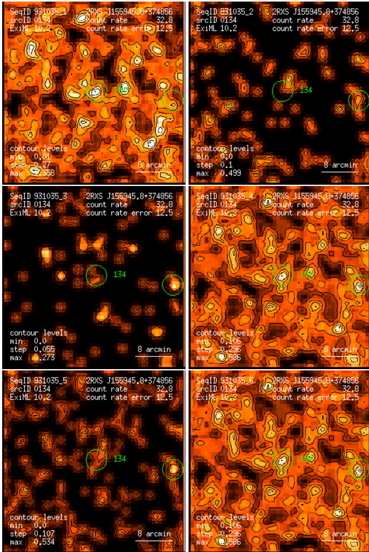
Figure 134: RASS 931035: detection 0134: band rate images, Gaussian filter: (1) PSPC channels 11 – 41, (2) 52 – 90, (3) 91 – 201, (4) 11 – 235, (5) 52 – 201, (6) 11 – 201. Broad band rates in counts/ks. Band rate contour levels in counts/ks/arcmin 2 .
