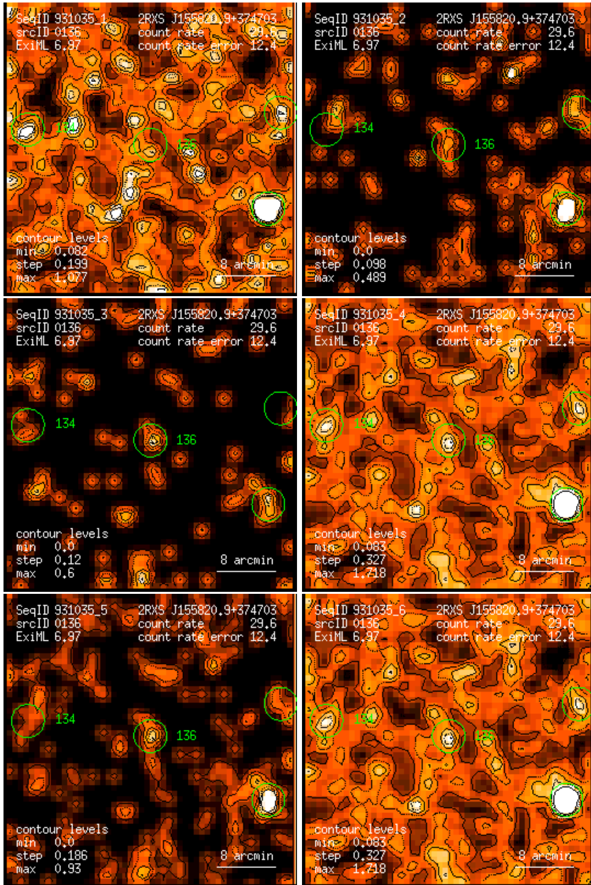
Figure 136: RASS 931035: detection 0136: band rate images, Gaussian filter: (1) PSPC channels 11 – 41, (2) 52 – 90, (3) 91 – 201, (4) 11 – 235, (5) 52 – 201, (6) 11 – 201. Broad band rates in counts/ks. Band rate contour levels in counts/ks/arcmin 2 .
