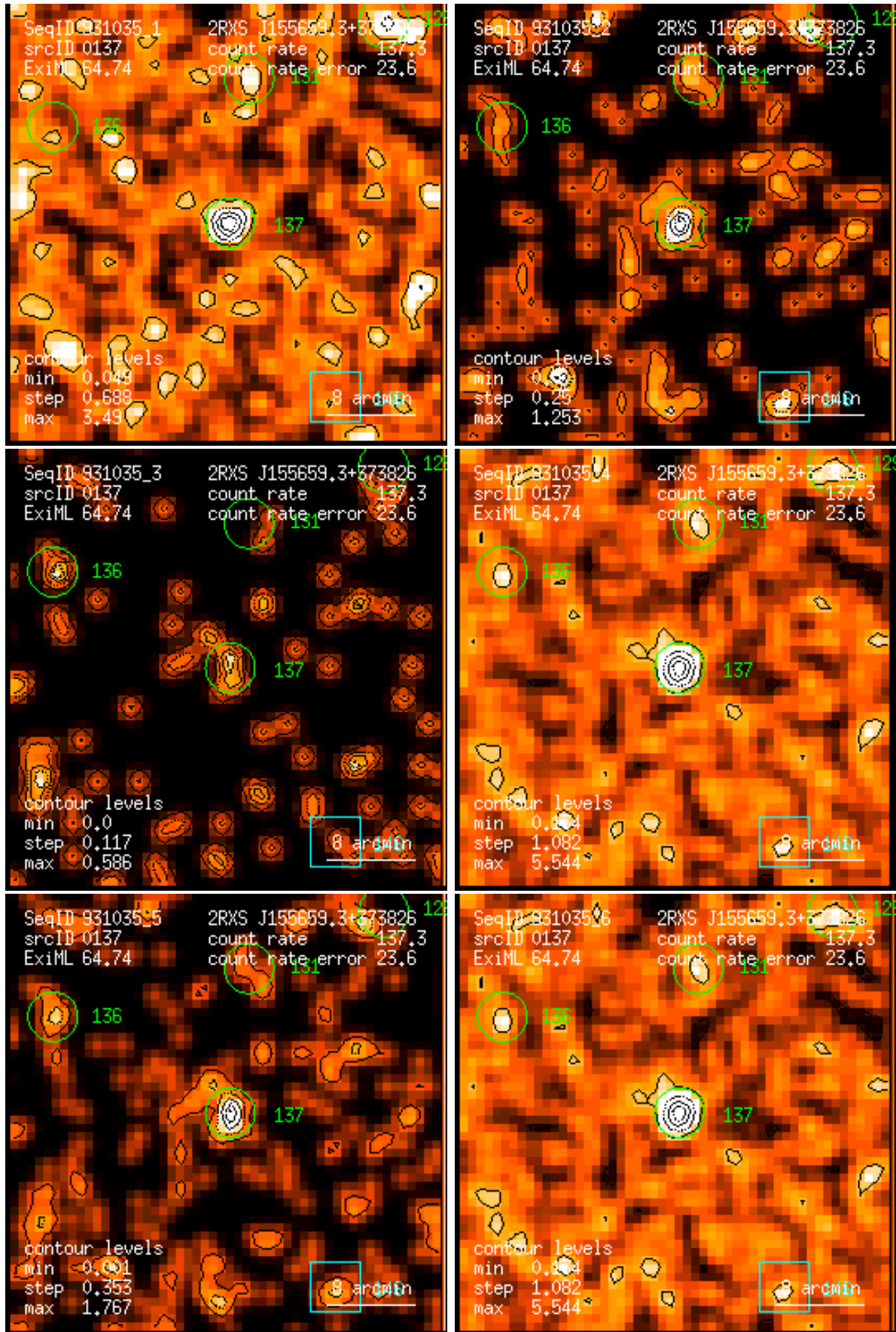
Figure 137: RASS 931035: detection 0137: band rate images, Gaussian filter: (1) PSPC channels 11 – 41, (2) 52 – 90, (3) 91 – 201, (4) 11 – 235, (5) 52 – 201, (6) 11 – 201. Broad band rates in counts/ks. Band rate contour levels in counts/ks/arcmin 2 .
