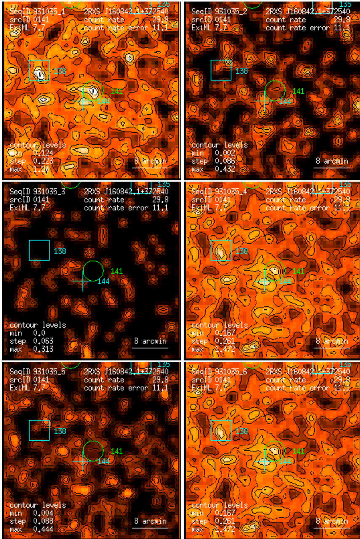
Figure 141: RASS 931035: detection 0141: band rate images, Gaussian filter: (1) PSPC channels 11 – 41, (2) 52 – 90, (3) 91 – 201, (4) 11 – 235, (5) 52 – 201, (6) 11 – 201. Broad band rates in counts/ks. Band rate contour levels in counts/ks/arcmin 2 .
