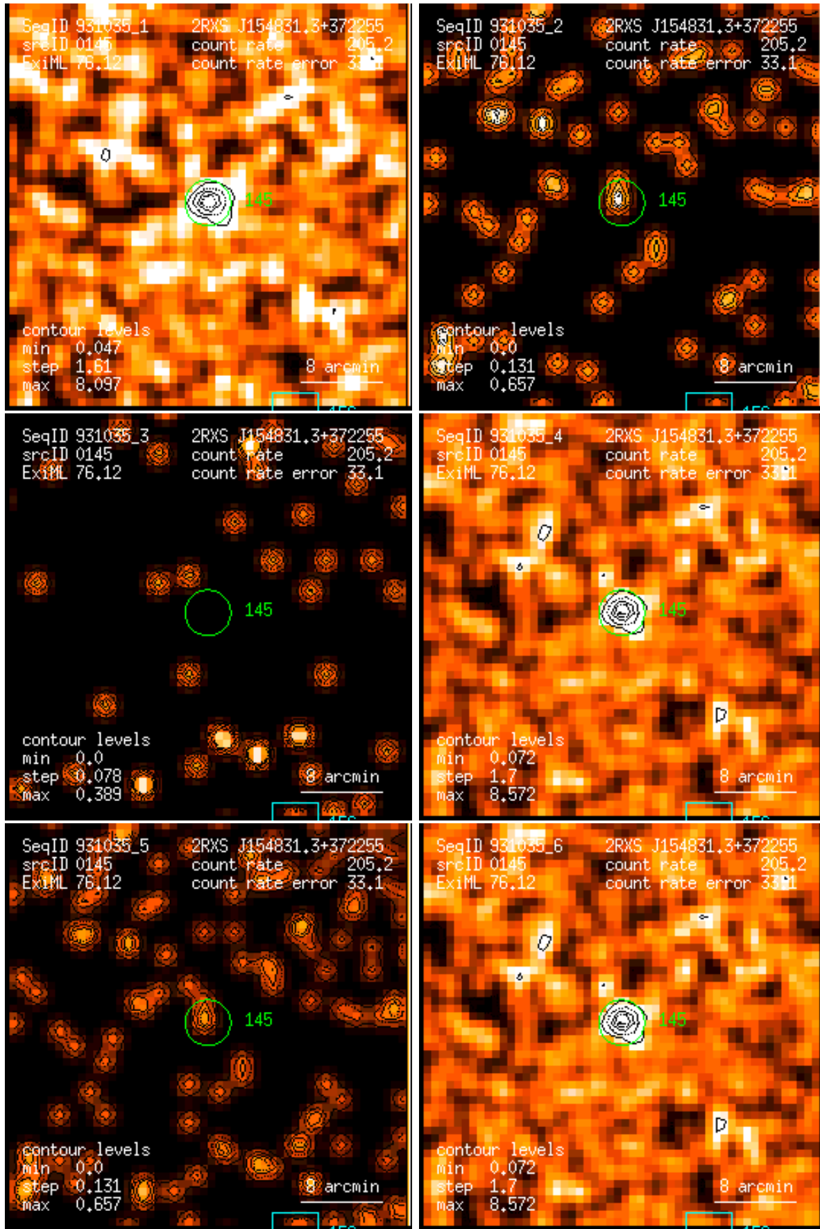
Figure 145: RASS 931035: detection 0145: band rate images, Gaussian filter: (1) PSPC channels 11 – 41, (2) 52 – 90, (3) 91 – 201, (4) 11 – 235, (5) 52 – 201, (6) 11 – 201. Broad band rates in counts/ks. Band rate contour levels in counts/ks/arcmin 2 .
