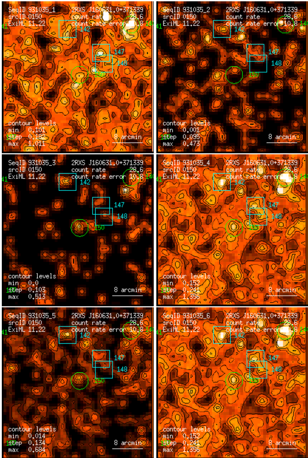
Figure 150: RASS 931035: detection 0150: band rate images, Gaussian filter: (1) PSPC channels 11 – 41, (2) 52 – 90, (3) 91 – 201, (4) 11 – 235, (5) 52 – 201, (6) 11 – 201. Broad band rates in counts/ks. Band rate contour levels in counts/ks/arcmin 2 .
