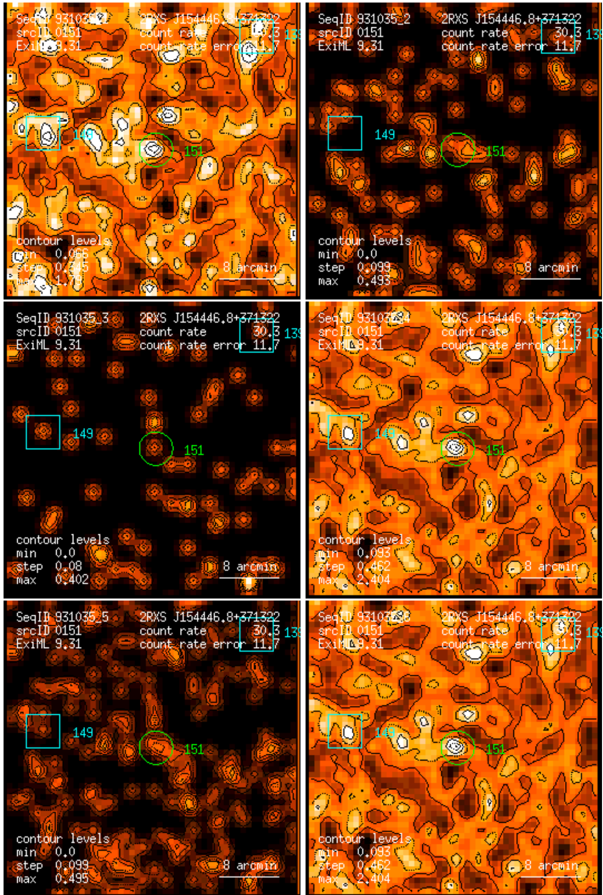
Figure 151: RASS 931035: detection 0151: band rate images, Gaussian filter: (1) PSPC channels 11 – 41, (2) 52 – 90, (3) 91 – 201, (4) 11 – 235, (5) 52 – 201, (6) 11 – 201. Broad band rates in counts/ks. Band rate contour levels in counts/ks/arcmin 2 .
