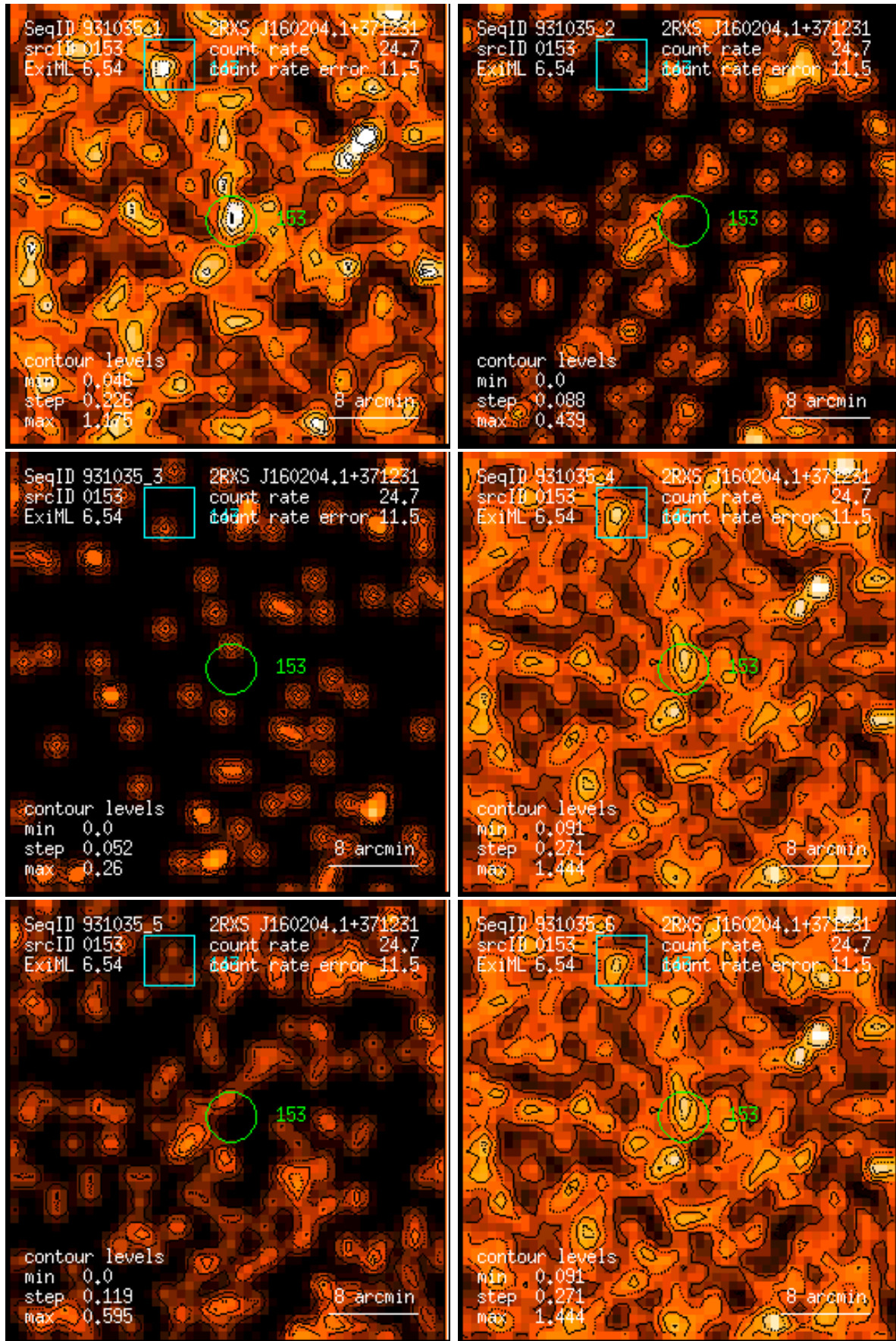
Figure 153: RASS 931035: detection 0153: band rate images, Gaussian filter: (1) PSPC channels 11 – 41, (2) 52 – 90, (3) 91 – 201, (4) 11 – 235, (5) 52 – 201, (6) 11 – 201. Broad band rates in counts/ks. Band rate contour levels in counts/ks/arcmin 2 .
