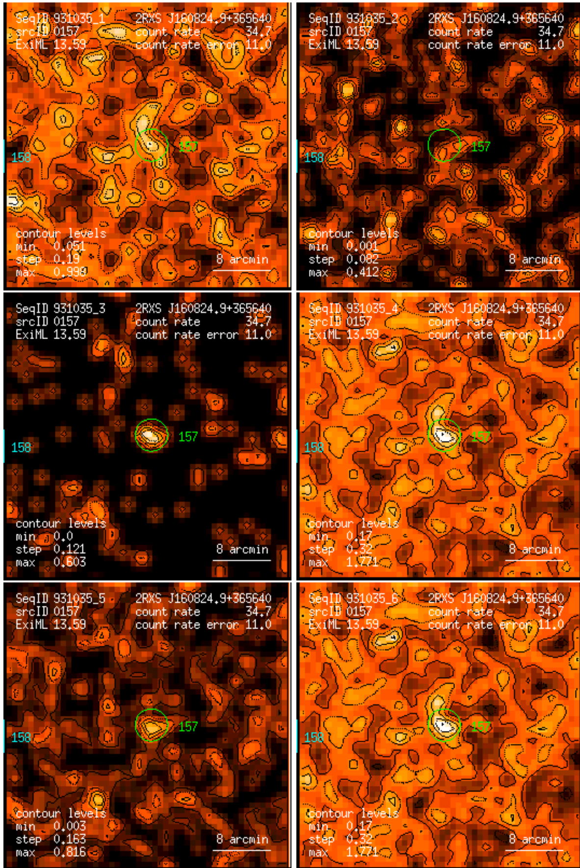
Figure 157: RASS 931035: detection 0157: band rate images, Gaussian filter: (1) PSPC channels 11 – 41, (2) 52 – 90, (3) 91 – 201, (4) 11 – 235, (5) 52 – 201, (6) 11 – 201. Broad band rates in counts/ks. Band rate contour levels in counts/ks/arcmin 2 .
