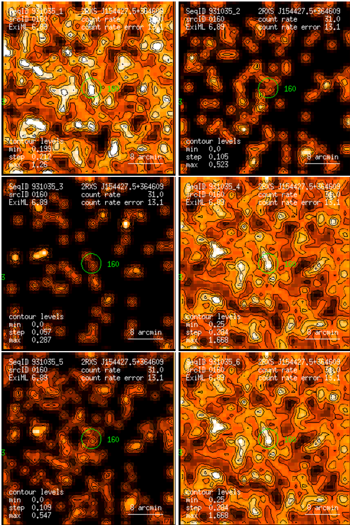
Figure 160: RASS 931035: detection 0160: band rate images, Gaussian filter: (1) PSPC channels 11 – 41, (2) 52 – 90, (3) 91 – 201, (4) 11 – 235, (5) 52 – 201, (6) 11 – 201. Broad band rates in counts/ks. Band rate contour levels in counts/ks/arcmin 2 .
