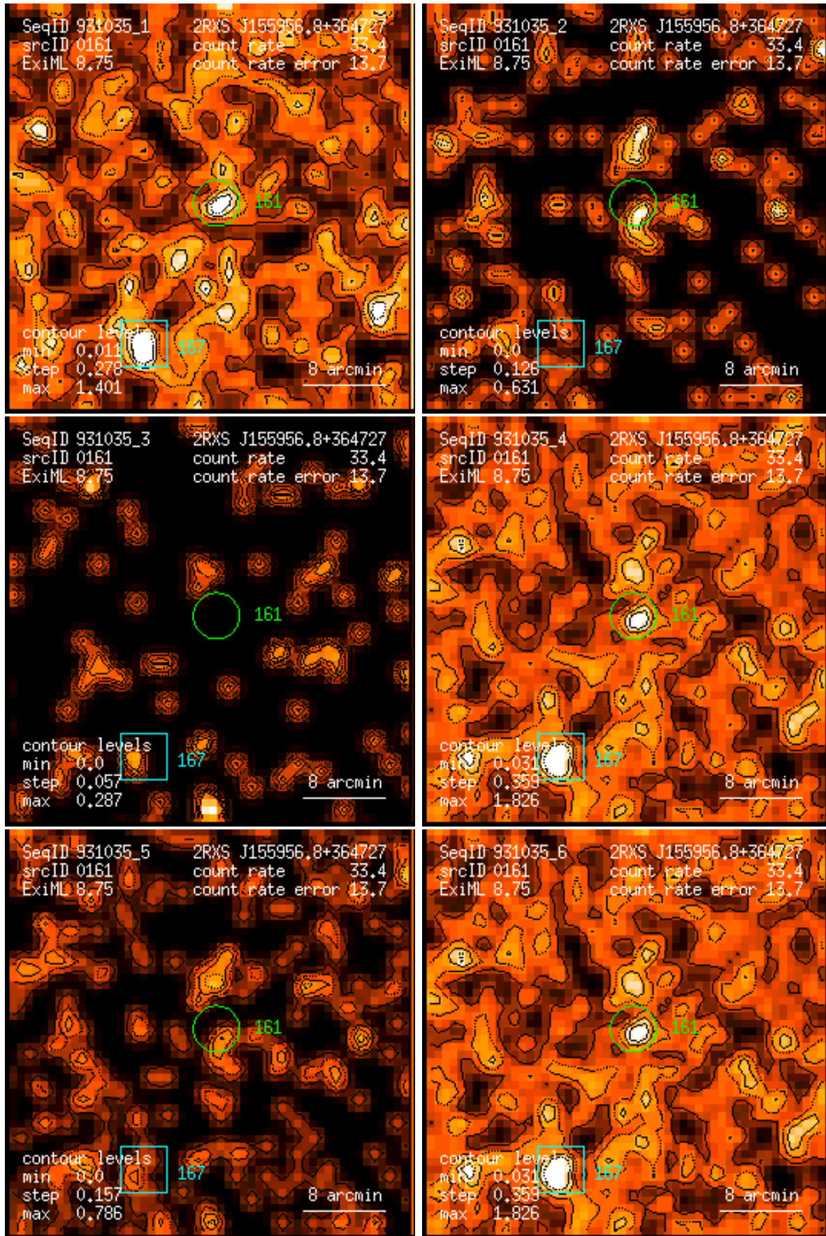
Figure 161: RASS 931035: detection 0161: band rate images, Gaussian filter: (1) PSPC channels 11 – 41, (2) 52 – 90, (3) 91 – 201, (4) 11 – 235, (5) 52 – 201, (6) 11 – 201. Broad band rates in counts/ks. Band rate contour levels in counts/ks/arcmin 2 .
