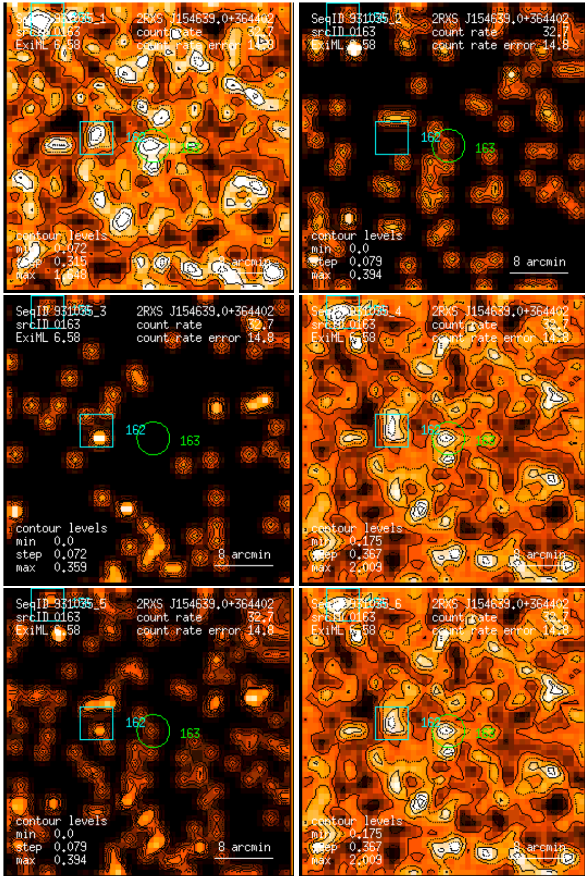
Figure 163: RASS 931035: detection 0163: band rate images, Gaussian filter: (1) PSPC channels 11 – 41, (2) 52 – 90, (3) 91 – 201, (4) 11 – 235, (5) 52 – 201, (6) 11 – 201. Broad band rates in counts/ks. Band rate contour levels in counts/ks/arcmin 2 .
