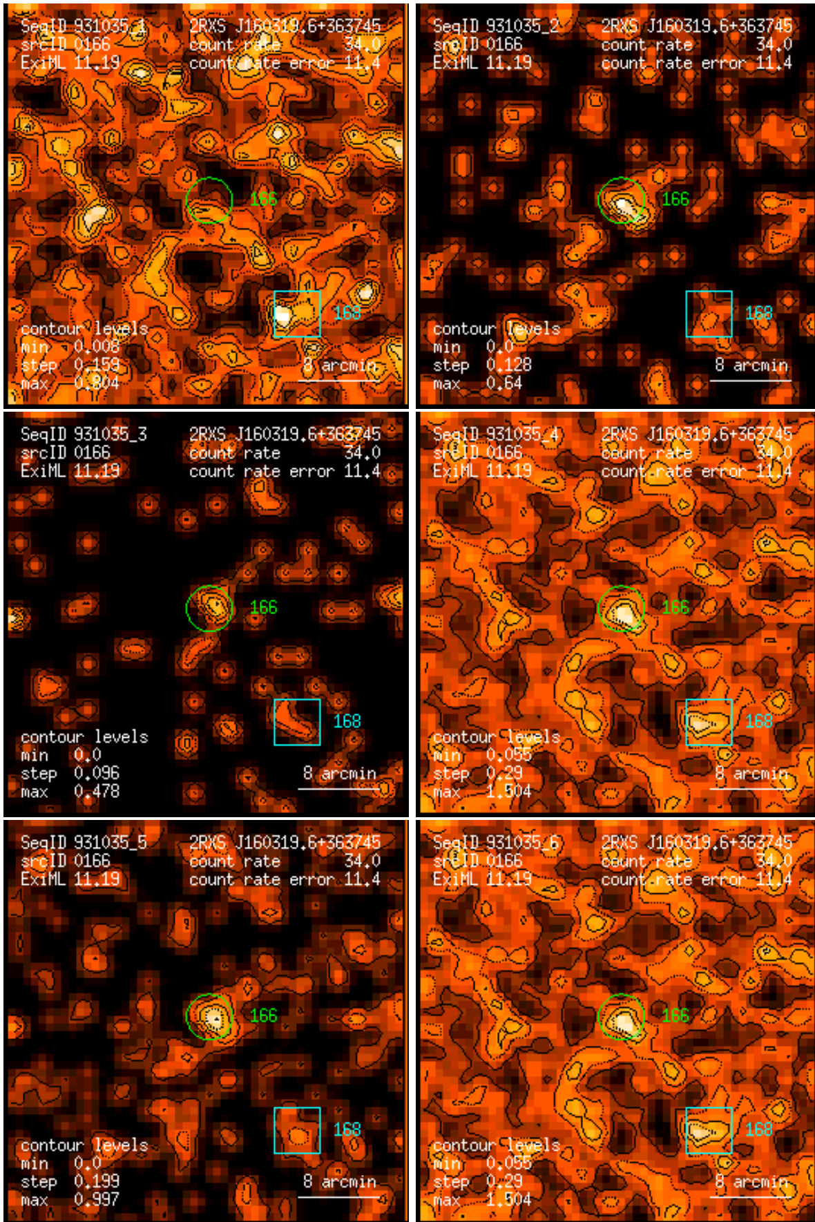
Figure 166: RASS 931035: detection 0166: band rate images, Gaussian filter: (1) PSPC channels 11 – 41, (2) 52 – 90, (3) 91 – 201, (4) 11 – 235, (5) 52 – 201, (6) 11 – 201. Broad band rates in counts/ks. Band rate contour levels in counts/ks/arcmin 2 .
