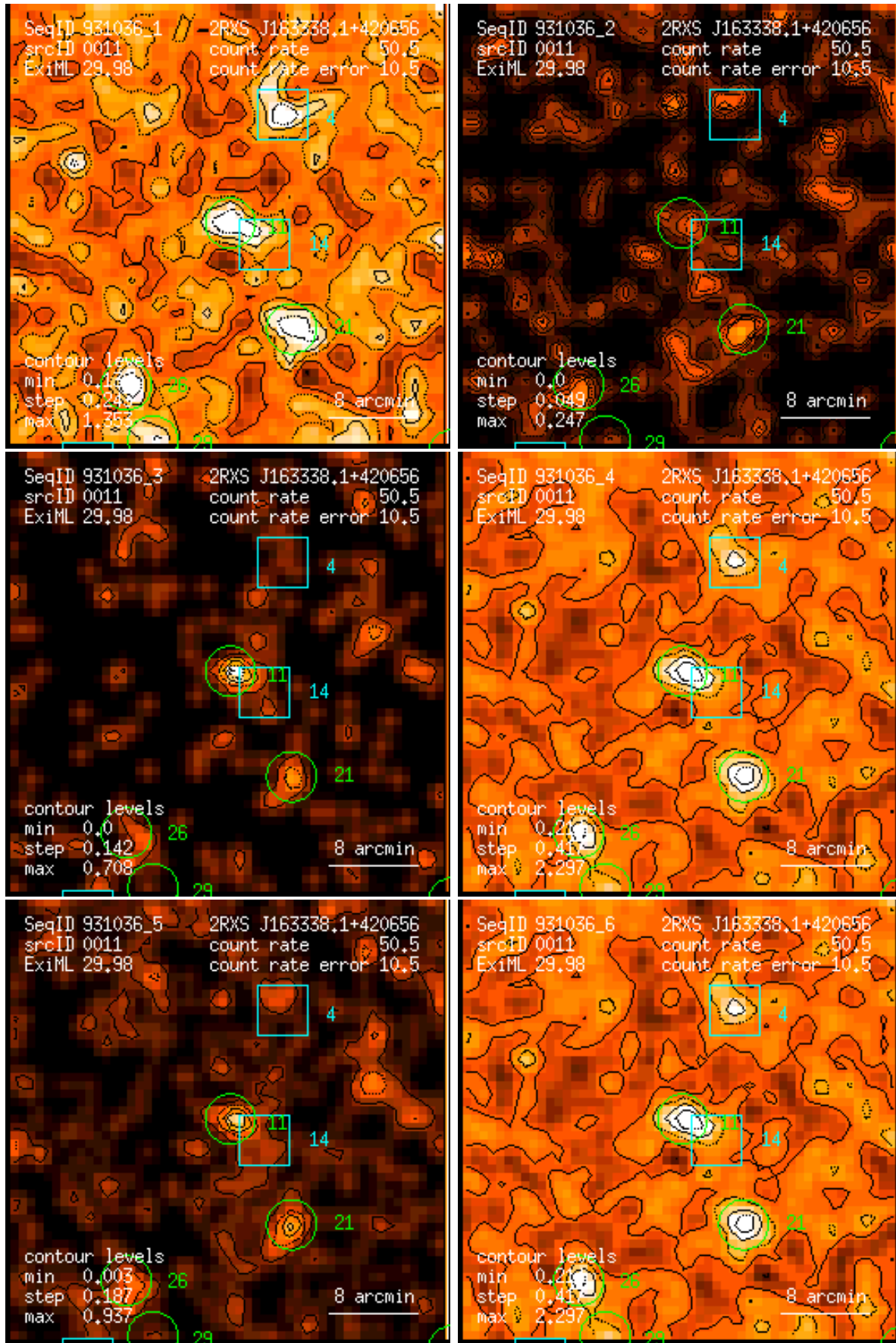
Figure 11: RASS 931036: detection 0011: band rate images, Gaussian filter: (1) PSPC channels 11 – 41, (2) 52 – 90, (3) 91 – 201, (4) 11 – 235, (5) 52 – 201, (6) 11 – 201. Broad band rates in counts/ks. Band rate contour levels in counts/ks/arcmin 2 .
