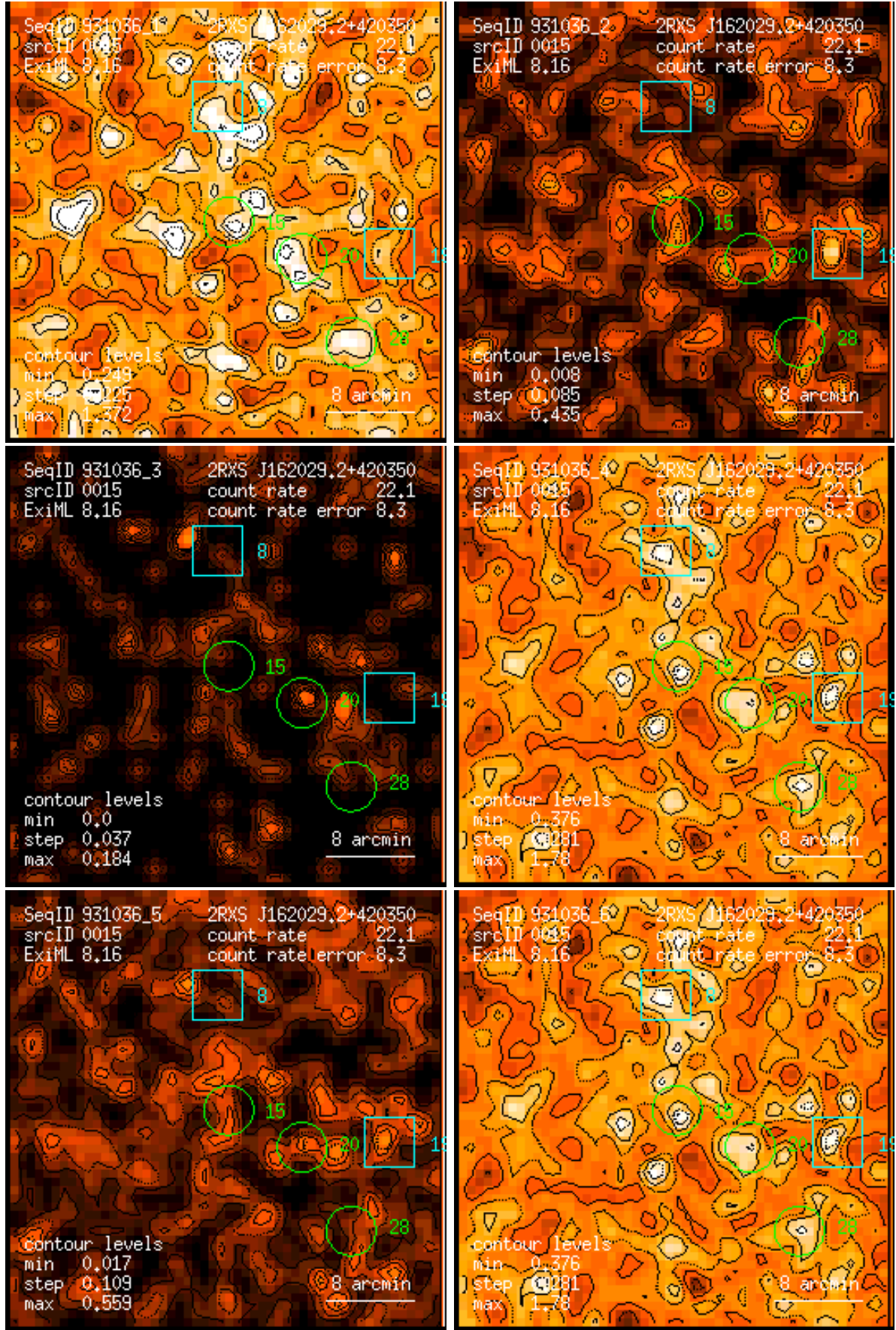
Figure 15: RASS 931036: detection 0015: band rate images, Gaussian filter: (1) PSPC channels 11 – 41, (2) 52 – 90, (3) 91 – 201, (4) 11 – 235, (5) 52 – 201, (6) 11 – 201. Broad band rates in counts/ks. Band rate contour levels in counts/ks/arcmin 2 .
