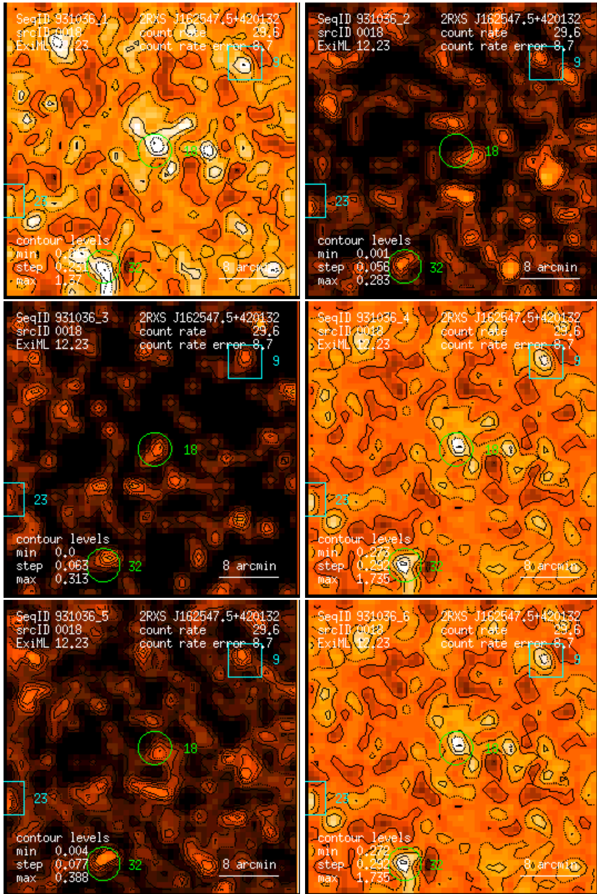
Figure 18: RASS 931036: detection 0018: band rate images, Gaussian filter: (1) PSPC channels 11 – 41, (2) 52 – 90, (3) 91 – 201, (4) 11 – 235, (5) 52 – 201, (6) 11 – 201. Broad band rates in counts/ks. Band rate contour levels in counts/ks/arcmin 2 .
