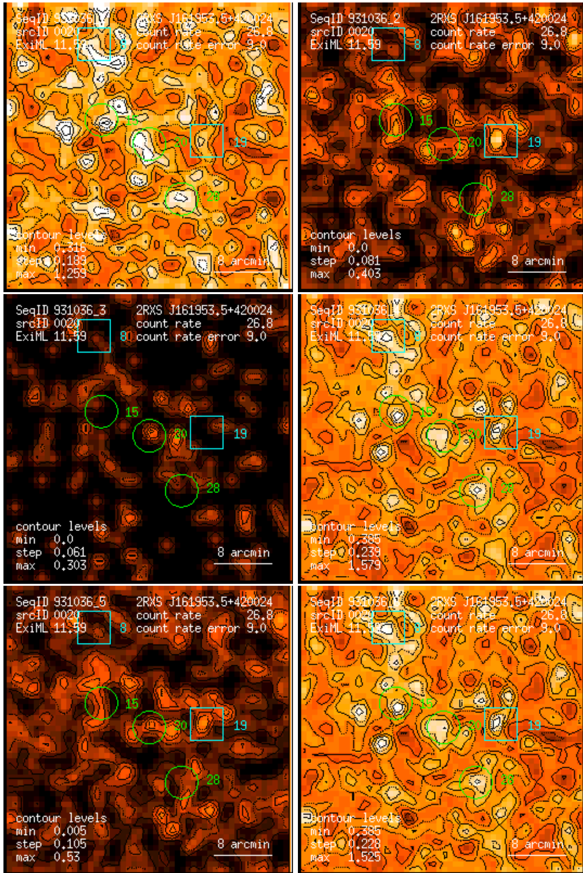
Figure 20: RASS 931036: detection 0020: band rate images, Gaussian filter: (1) PSPC channels 11 – 41, (2) 52 – 90, (3) 91 – 201, (4) 11 – 235, (5) 52 – 201, (6) 11 – 201. Broad band rates in counts/ks. Band rate contour levels in counts/ks/arcmin 2 .
