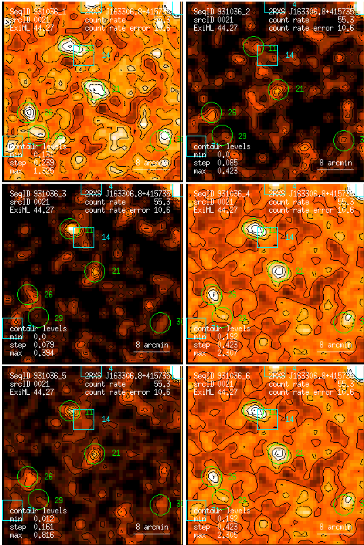
Figure 21: RASS 931036: detection 0021: band rate images, Gaussian filter: (1) PSPC channels 11 – 41, (2) 52 – 90, (3) 91 – 201, (4) 11 – 235, (5) 52 – 201, (6) 11 – 201. Broad band rates in counts/ks. Band rate contour levels in counts/ks/arcmin 2 .
