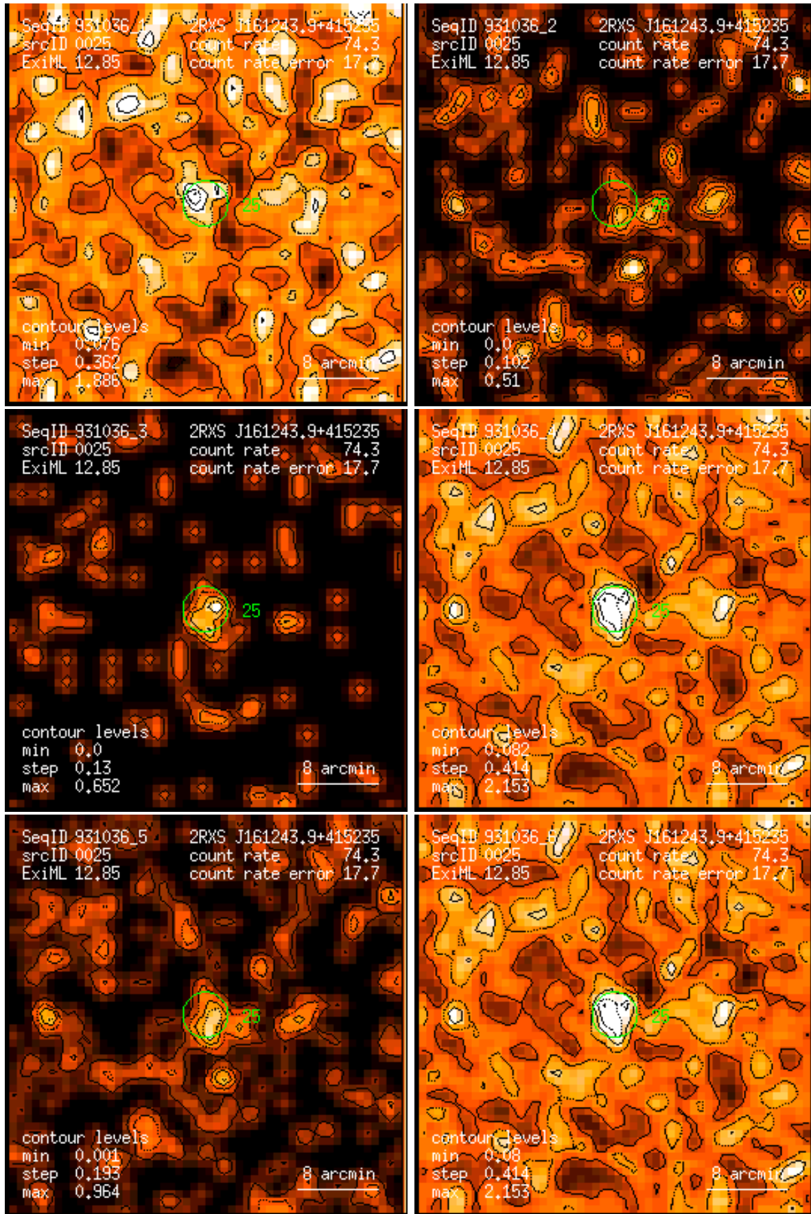
Figure 25: RASS 931036: detection 0025: band rate images, Gaussian filter: (1) PSPC channels 11 – 41, (2) 52 – 90, (3) 91 – 201, (4) 11 – 235, (5) 52 – 201, (6) 11 – 201. Broad band rates in counts/ks. Band rate contour levels in counts/ks/arcmin 2 .
