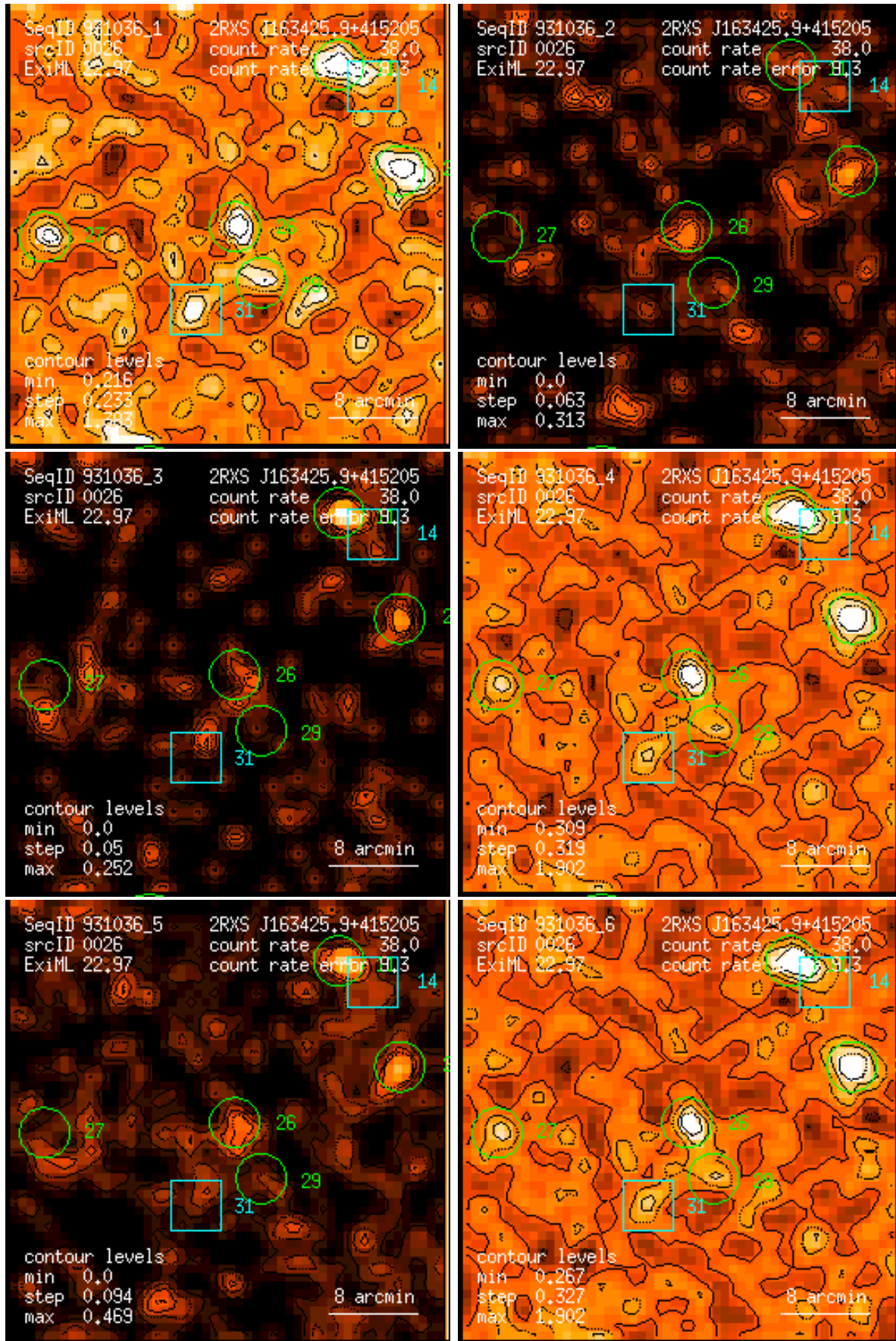
Figure 26: RASS 931036: detection 0026: band rate images, Gaussian filter: (1) PSPC channels 11 – 41, (2) 52 – 90, (3) 91 – 201, (4) 11 – 235, (5) 52 – 201, (6) 11 – 201. Broad band rates in counts/ks. Band rate contour levels in counts/ks/arcmin 2 .
