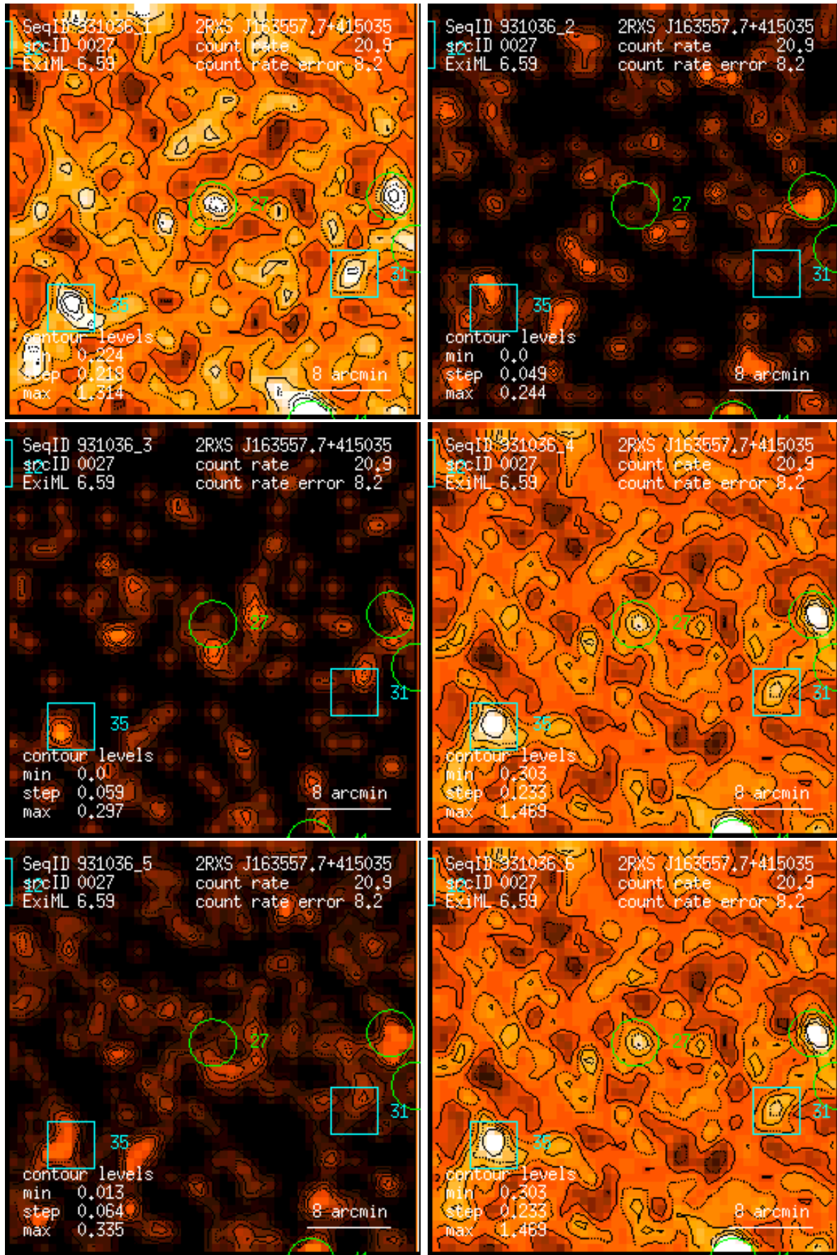
Figure 27: RASS 931036: detection 0027: band rate images, Gaussian filter: (1) PSPC channels 11 – 41, (2) 52 – 90, (3) 91 – 201, (4) 11 – 235, (5) 52 – 201, (6) 11 – 201. Broad band rates in counts/ks. Band rate contour levels in counts/ks/arcmin 2 .
