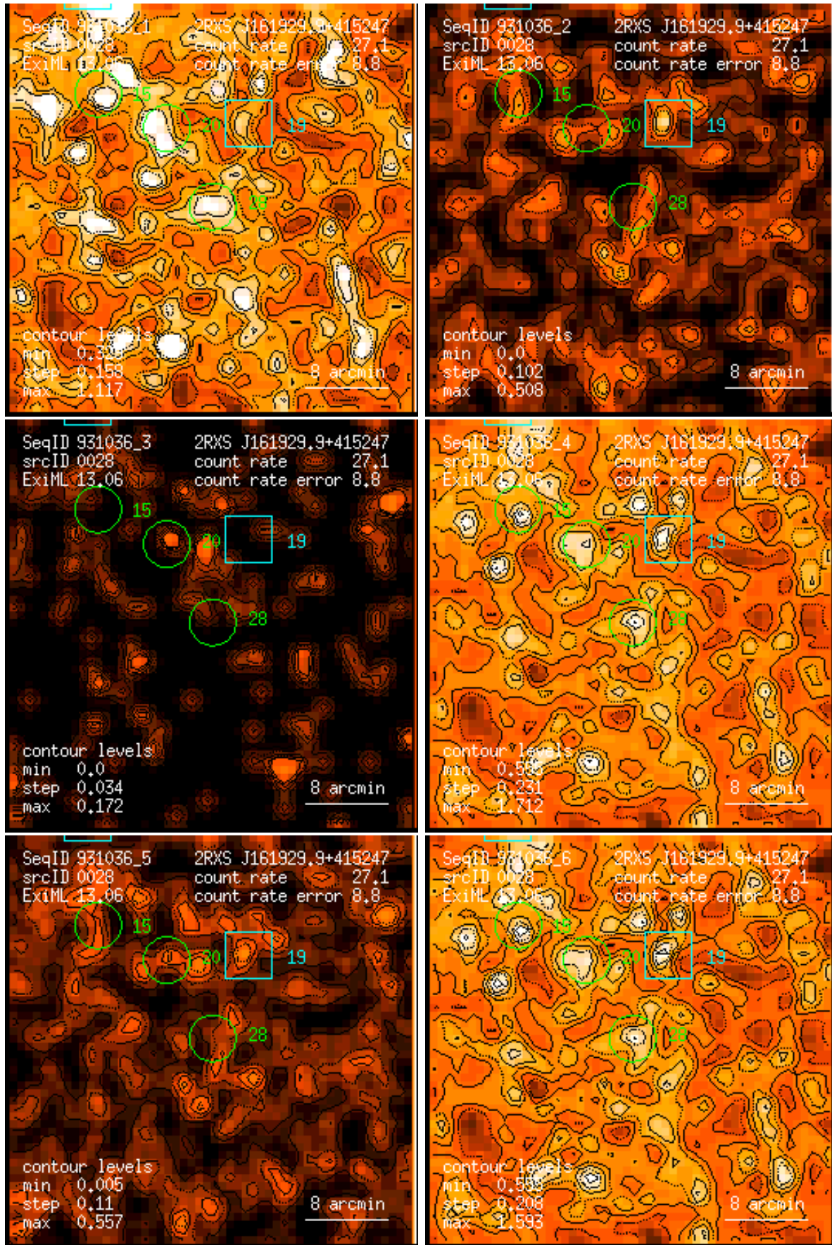
Figure 28: RASS 931036: detection 0028: band rate images, Gaussian filter: (1) PSPC channels 11 – 41, (2) 52 – 90, (3) 91 – 201, (4) 11 – 235, (5) 52 – 201, (6) 11 – 201. Broad band rates in counts/ks. Band rate contour levels in counts/ks/arcmin 2 .
