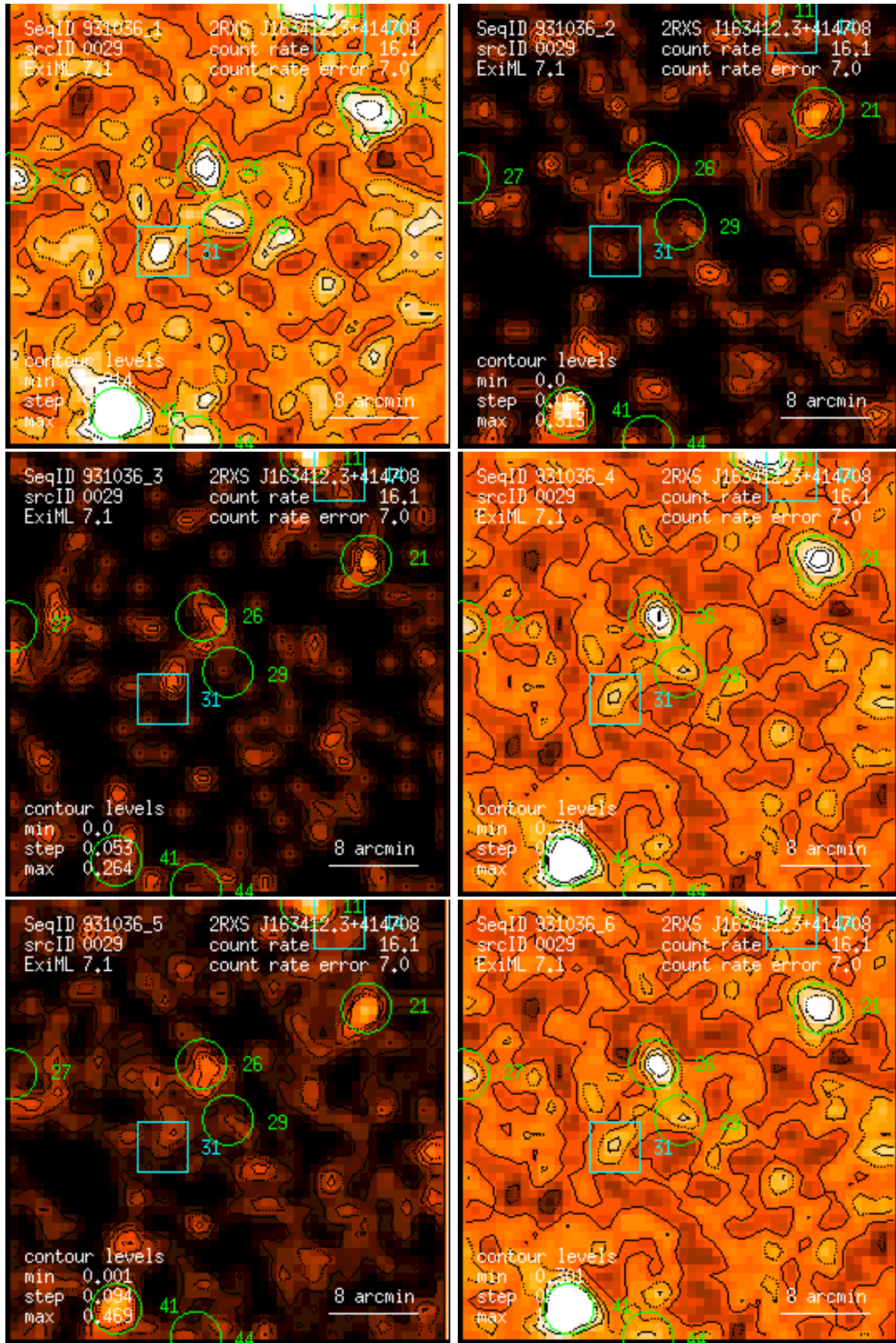
Figure 29: RASS 931036: detection 0029: band rate images, Gaussian filter: (1) PSPC channels 11 – 41, (2) 52 – 90, (3) 91 – 201, (4) 11 – 235, (5) 52 – 201, (6) 11 – 201. Broad band rates in counts/ks. Band rate contour levels in counts/ks/arcmin 2 .
