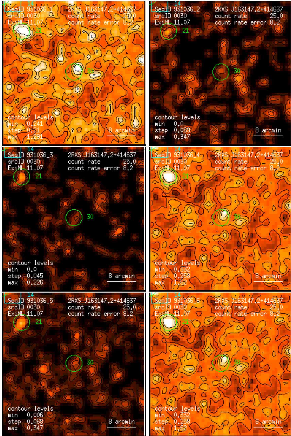
Figure 30: RASS 931036: detection 0030: band rate images, Gaussian filter: (1) PSPC channels 11 – 41, (2) 52 – 90, (3) 91 – 201, (4) 11 – 235, (5) 52 – 201, (6) 11 – 201. Broad band rates in counts/ks. Band rate contour levels in counts/ks/arcmin 2 .
