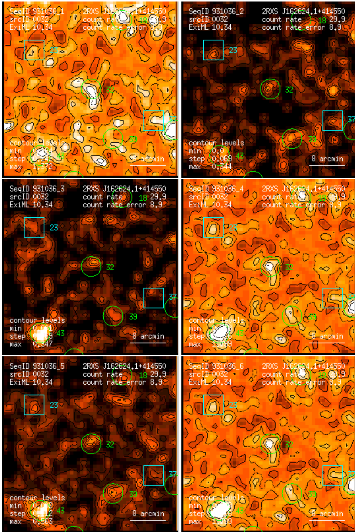
Figure 32: RASS 931036: detection 0032: band rate images, Gaussian filter: (1) PSPC channels 11 – 41, (2) 52 – 90, (3) 91 – 201, (4) 11 – 235, (5) 52 – 201, (6) 11 – 201. Broad band rates in counts/ks. Band rate contour levels in counts/ks/arcmin 2 .
