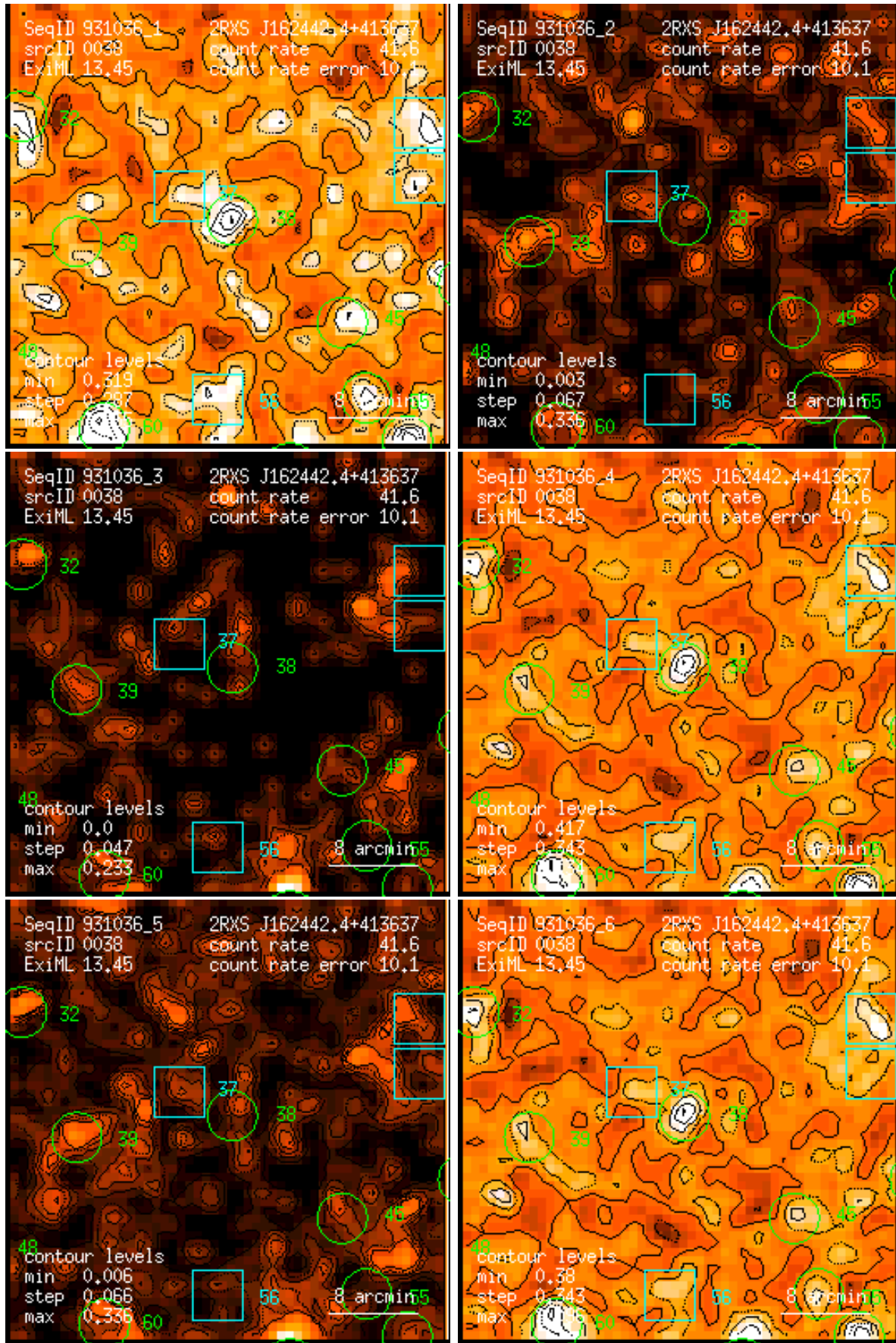
Figure 38: RASS 931036: detection 0038: band rate images, Gaussian filter: (1) PSPC channels 11 – 41, (2) 52 – 90, (3) 91 – 201, (4) 11 – 235, (5) 52 – 201, (6) 11 – 201. Broad band rates in counts/ks. Band rate contour levels in counts/ks/arcmin 2 .
