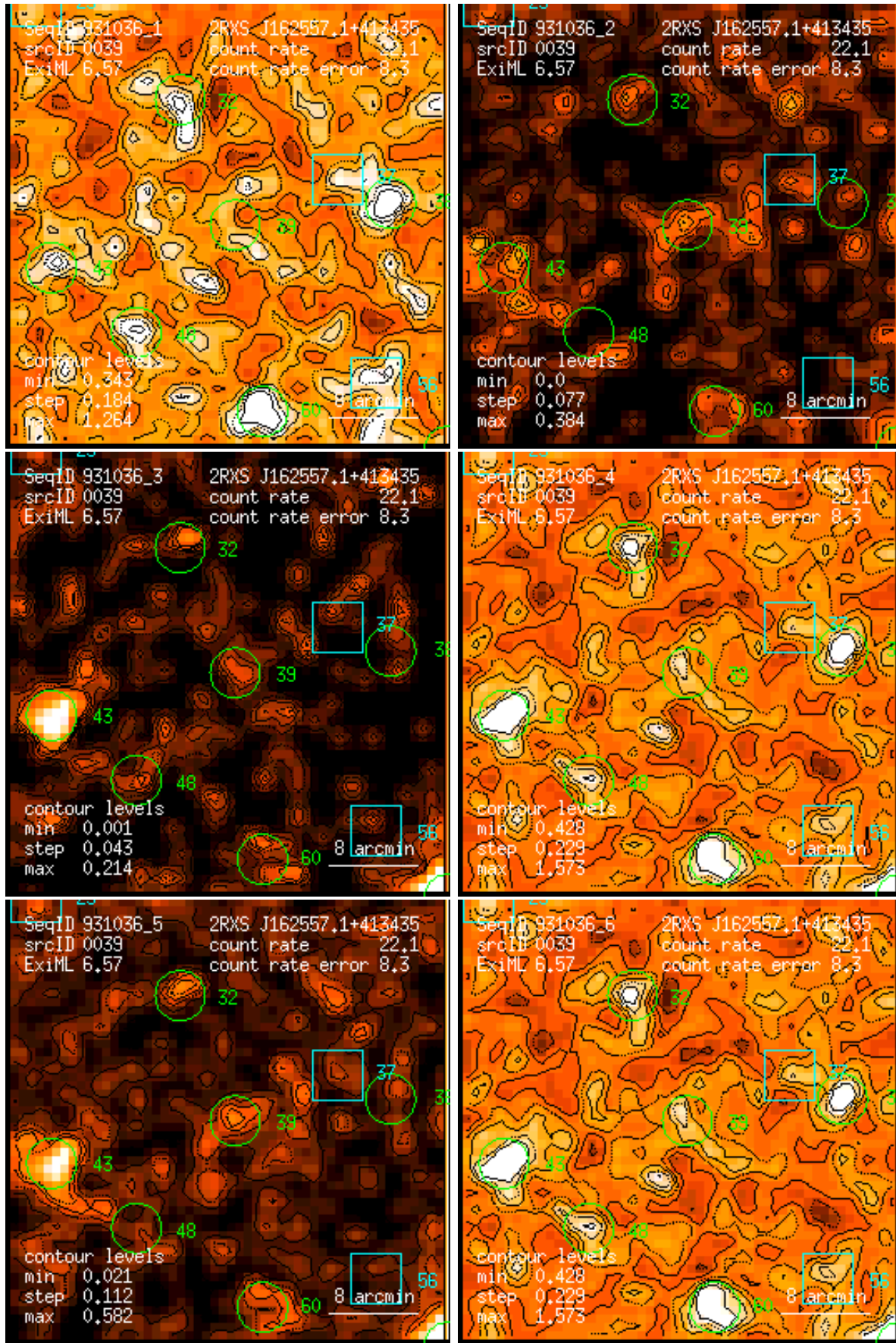
Figure 39: RASS 931036: detection 0039: band rate images, Gaussian filter: (1) PSPC channels 11 – 41, (2) 52 – 90, (3) 91 – 201, (4) 11 – 235, (5) 52 – 201, (6) 11 – 201. Broad band rates in counts/ks. Band rate contour levels in counts/ks/arcmin 2 .
