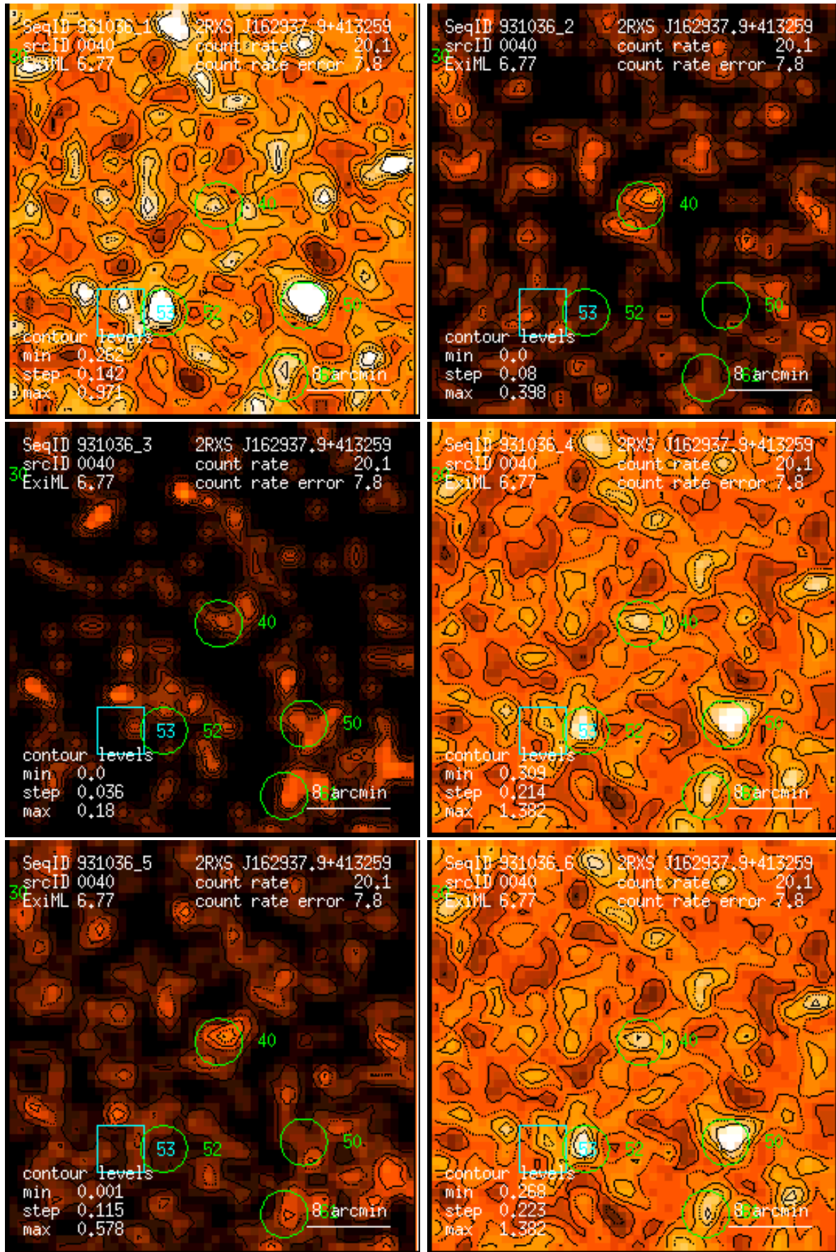
Figure 40: RASS 931036: detection 0040: band rate images, Gaussian filter: (1) PSPC channels 11 – 41, (2) 52 – 90, (3) 91 – 201, (4) 11 – 235, (5) 52 – 201, (6) 11 – 201. Broad band rates in counts/ks. Band rate contour levels in counts/ks/arcmin 2 .
