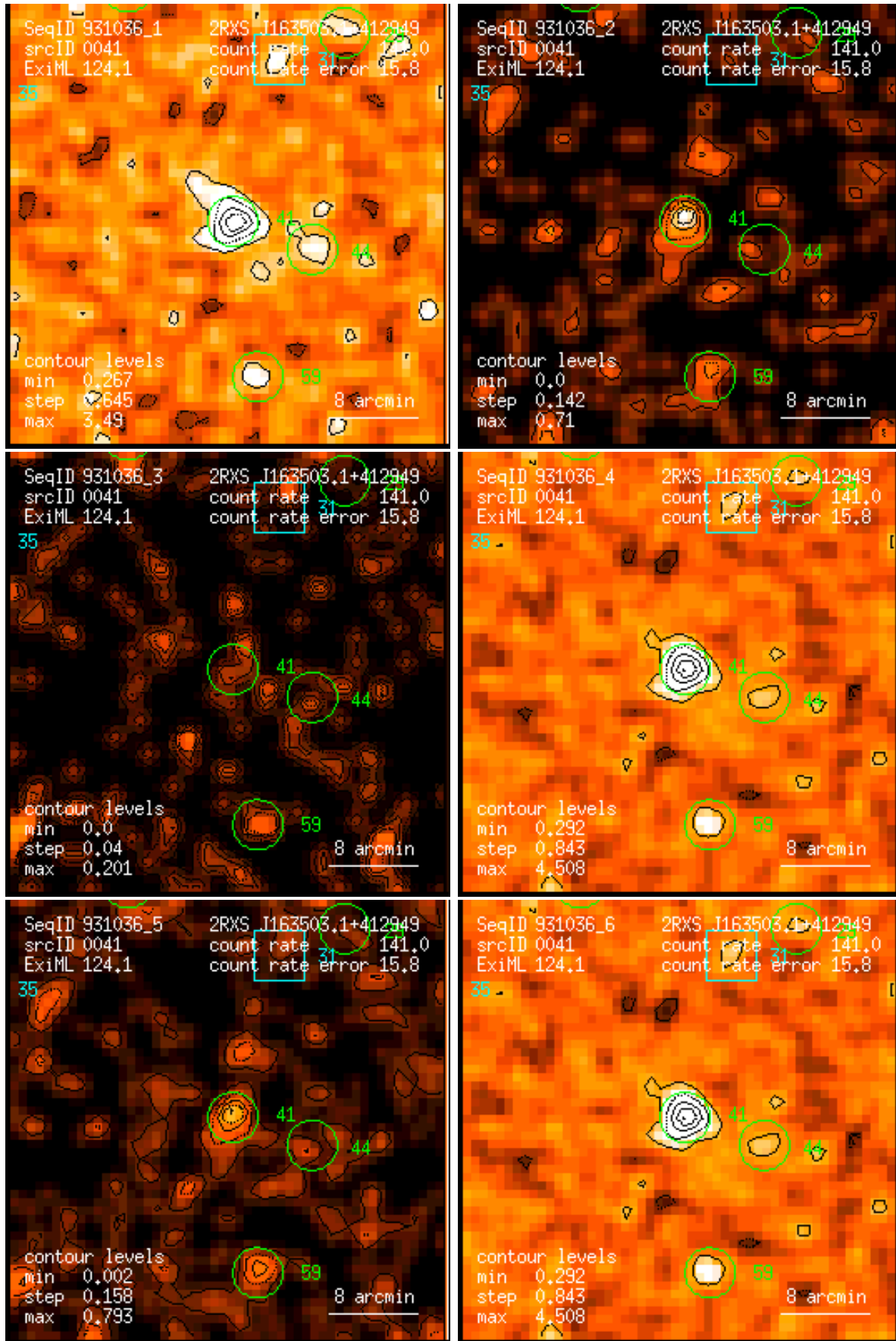
Figure 41: RASS 931036: detection 0041: band rate images, Gaussian filter: (1) PSPC channels 11 – 41, (2) 52 – 90, (3) 91 – 201, (4) 11 – 235, (5) 52 – 201, (6) 11 – 201. Broad band rates in counts/ks. Band rate contour levels in counts/ks/arcmin 2 .
