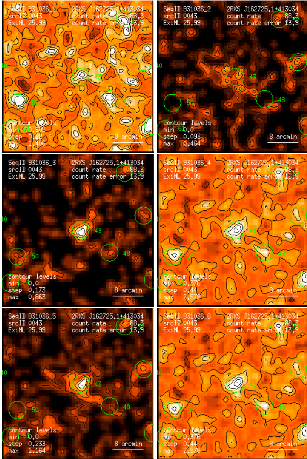
Figure 43: RASS 931036: detection 0043: band rate images, Gaussian filter: (1) PSPC channels 11 – 41, (2) 52 – 90, (3) 91 – 201, (4) 11 – 235, (5) 52 – 201, (6) 11 – 201. Broad band rates in counts/ks. Band rate contour levels in counts/ks/arcmin 2 .
