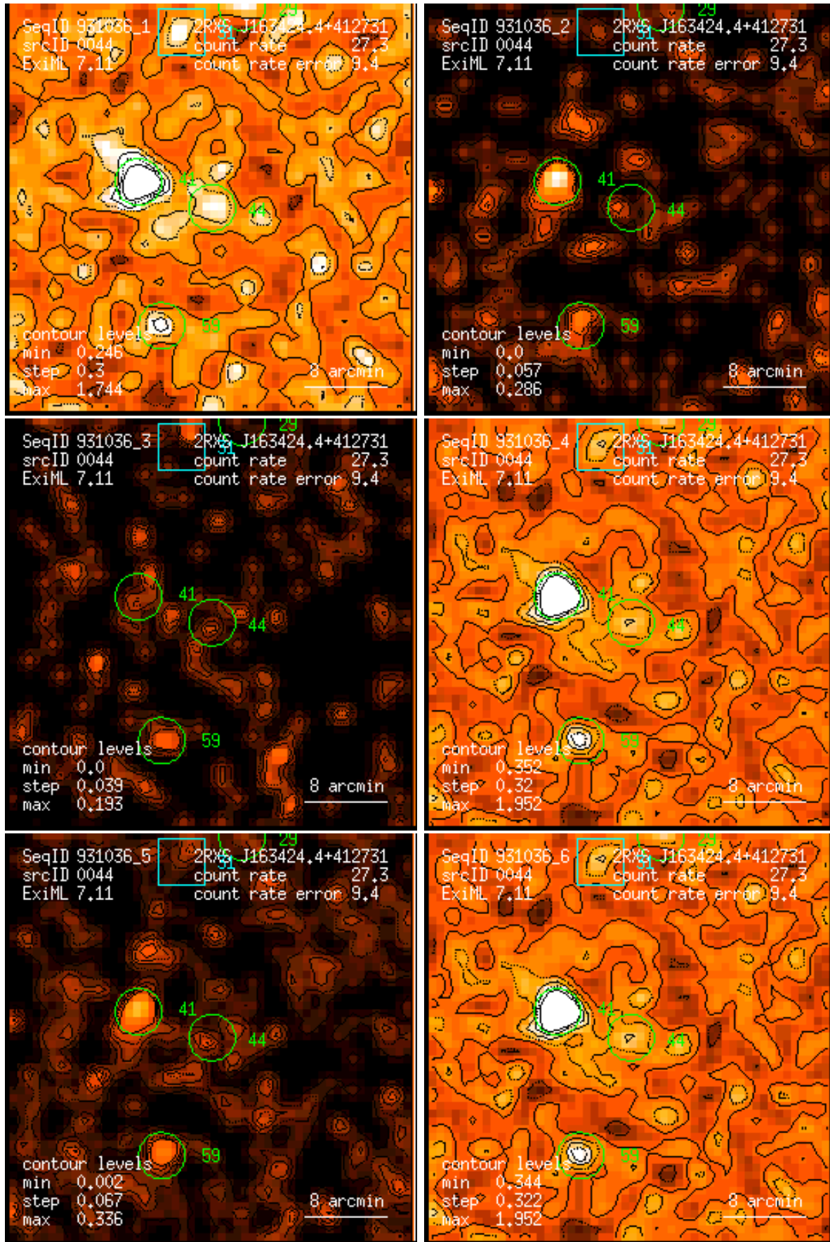
Figure 44: RASS 931036: detection 0044: band rate images, Gaussian filter: (1) PSPC channels 11 – 41, (2) 52 – 90, (3) 91 – 201, (4) 11 – 235, (5) 52 – 201, (6) 11 – 201. Broad band rates in counts/ks. Band rate contour levels in counts/ks/arcmin 2 .
