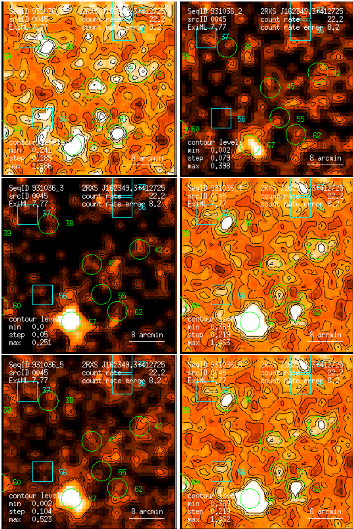
Figure 45: RASS 931036: detection 0045: band rate images, Gaussian filter: (1) PSPC channels 11 – 41, (2) 52 – 90, (3) 91 – 201, (4) 11 – 235, (5) 52 – 201, (6) 11 – 201. Broad band rates in counts/ks. Band rate contour levels in counts/ks/arcmin 2 .
