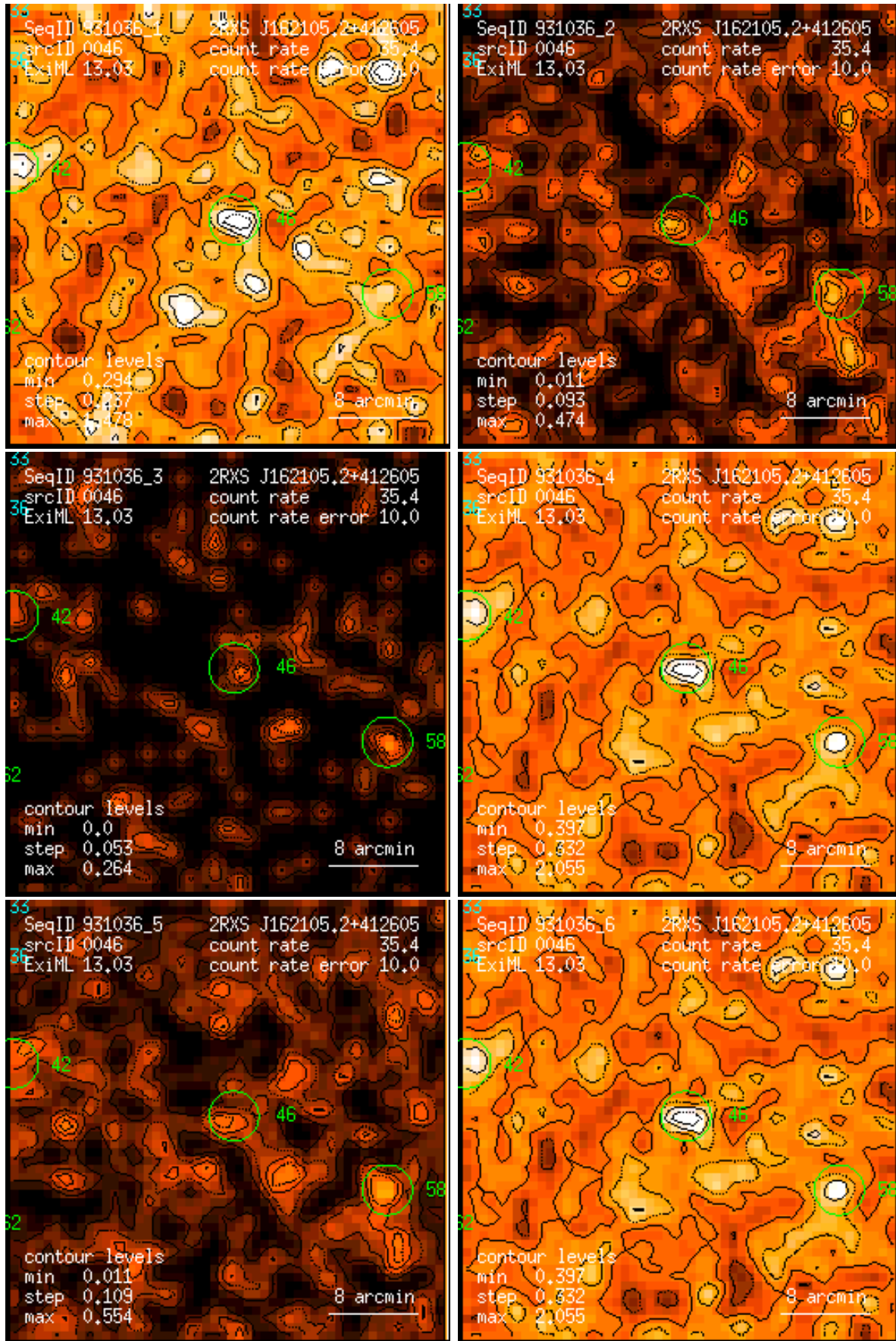
Figure 46: RASS 931036: detection 0046: band rate images, Gaussian filter: (1) PSPC channels 11 – 41, (2) 52 – 90, (3) 91 – 201, (4) 11 – 235, (5) 52 – 201, (6) 11 – 201. Broad band rates in counts/ks. Band rate contour levels in counts/ks/arcmin 2 .
