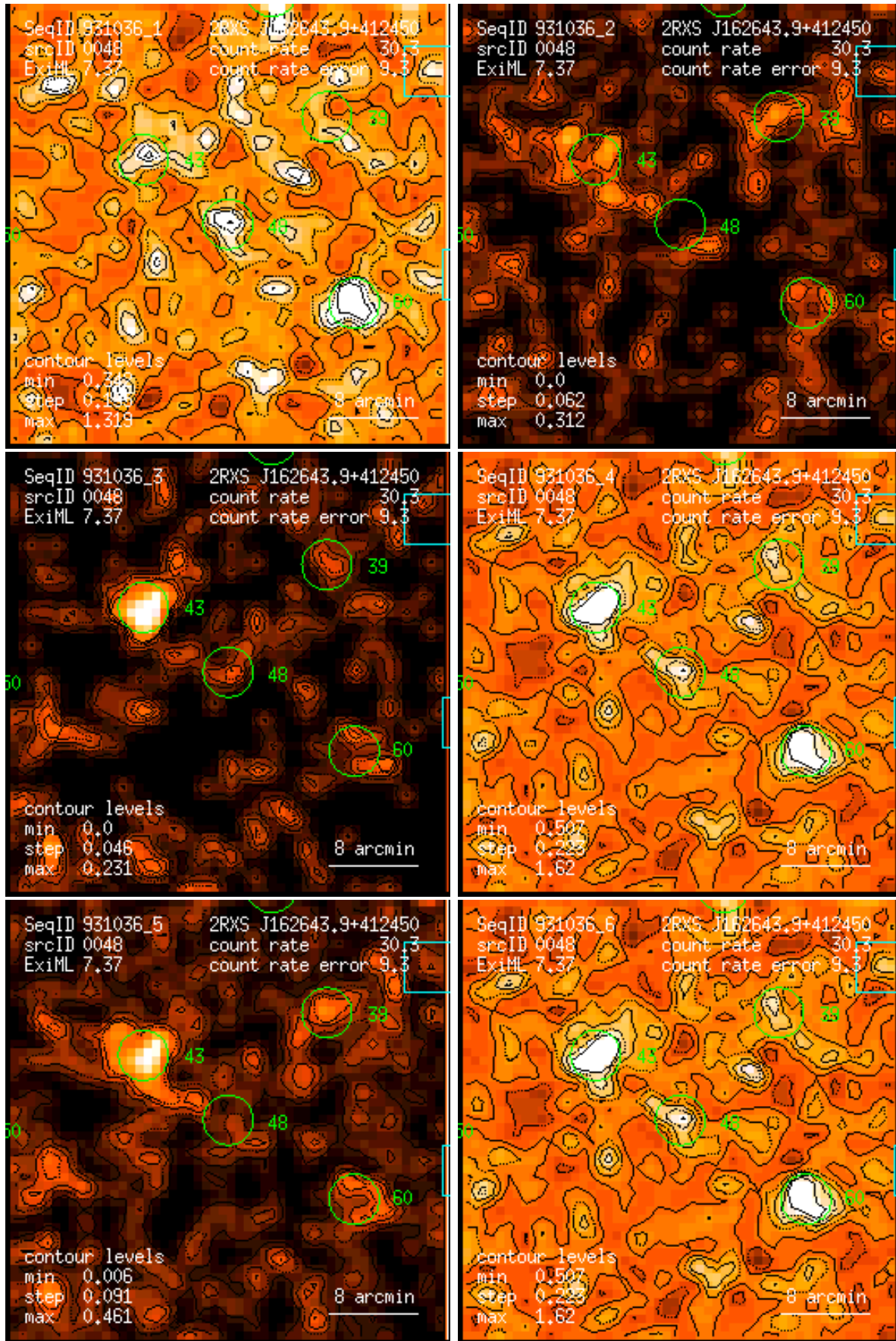
Figure 48: RASS 931036: detection 0048: band rate images, Gaussian filter: (1) PSPC channels 11 – 41, (2) 52 – 90, (3) 91 – 201, (4) 11 – 235, (5) 52 – 201, (6) 11 – 201. Broad band rates in counts/ks. Band rate contour levels in counts/ks/arcmin 2 .
