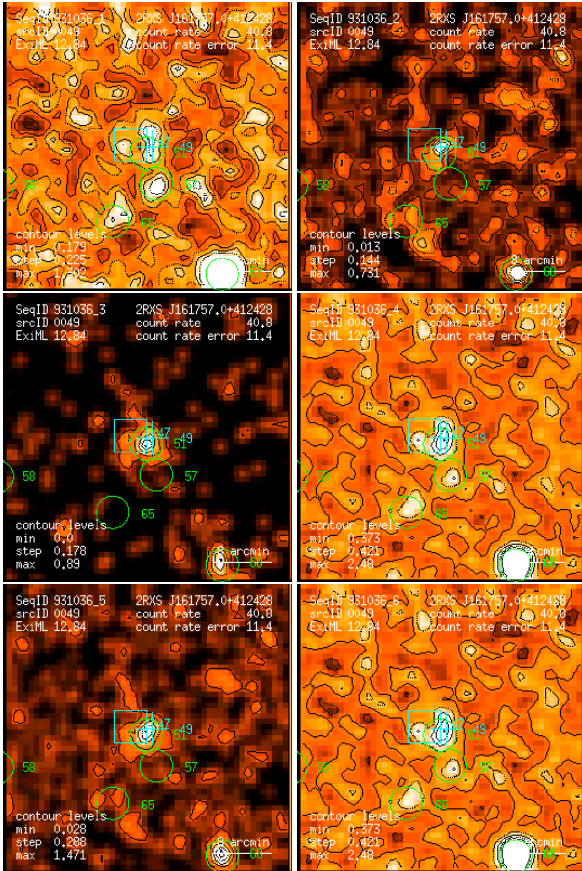
Figure 49: RASS 931036: detection 0049: band rate images, Gaussian filter: (1) PSPC channels 11 – 41, (2) 52 – 90, (3) 91 – 201, (4) 11 – 235, (5) 52 – 201, (6) 11 – 201. Broad band rates in counts/ks. Band rate contour levels in counts/ks/arcmin 2 .
