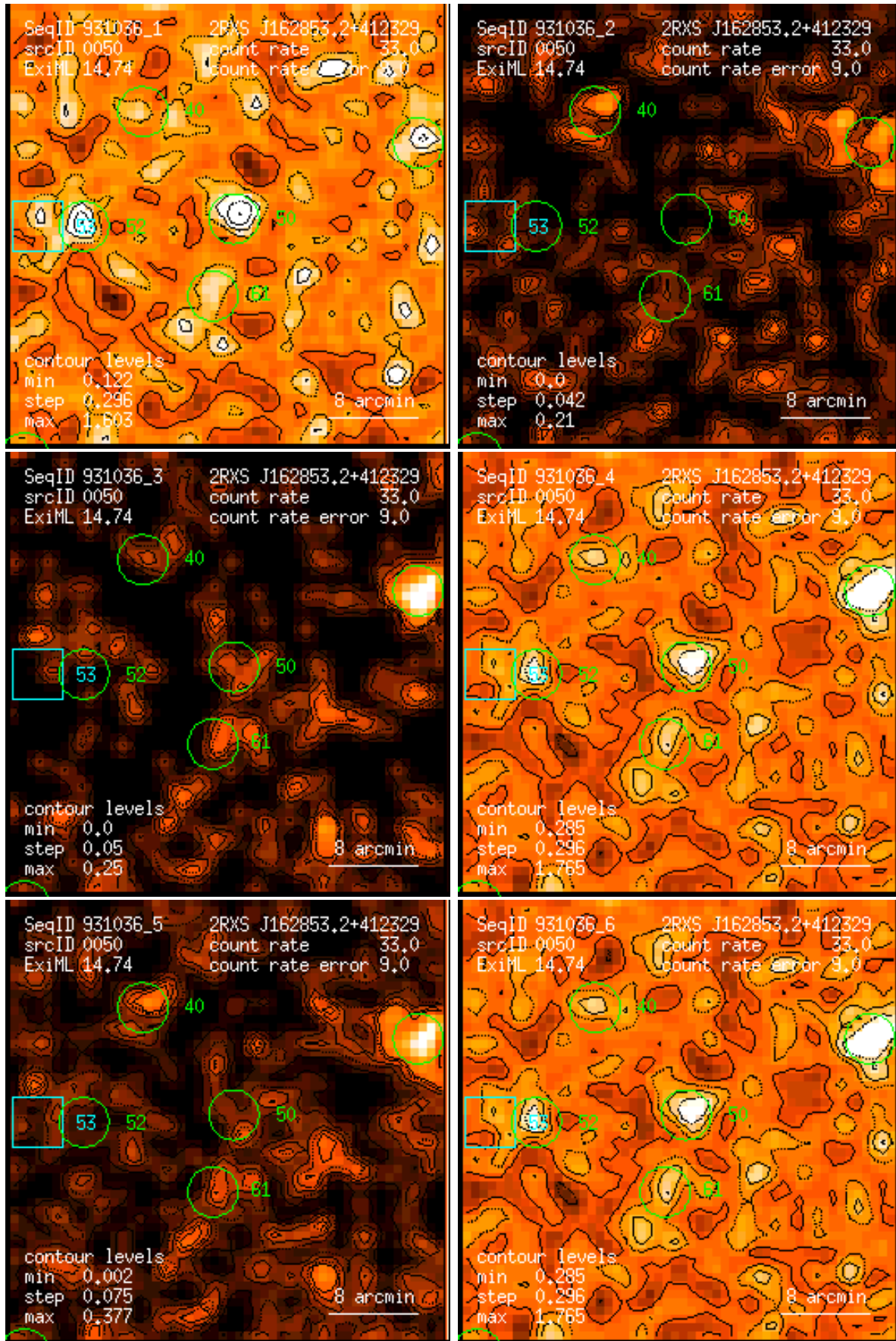
Figure 50: RASS 931036: detection 0050: band rate images, Gaussian filter: (1) PSPC channels 11 – 41, (2) 52 – 90, (3) 91 – 201, (4) 11 – 235, (5) 52 – 201, (6) 11 – 201. Broad band rates in counts/ks. Band rate contour levels in counts/ks/arcmin 2 .
