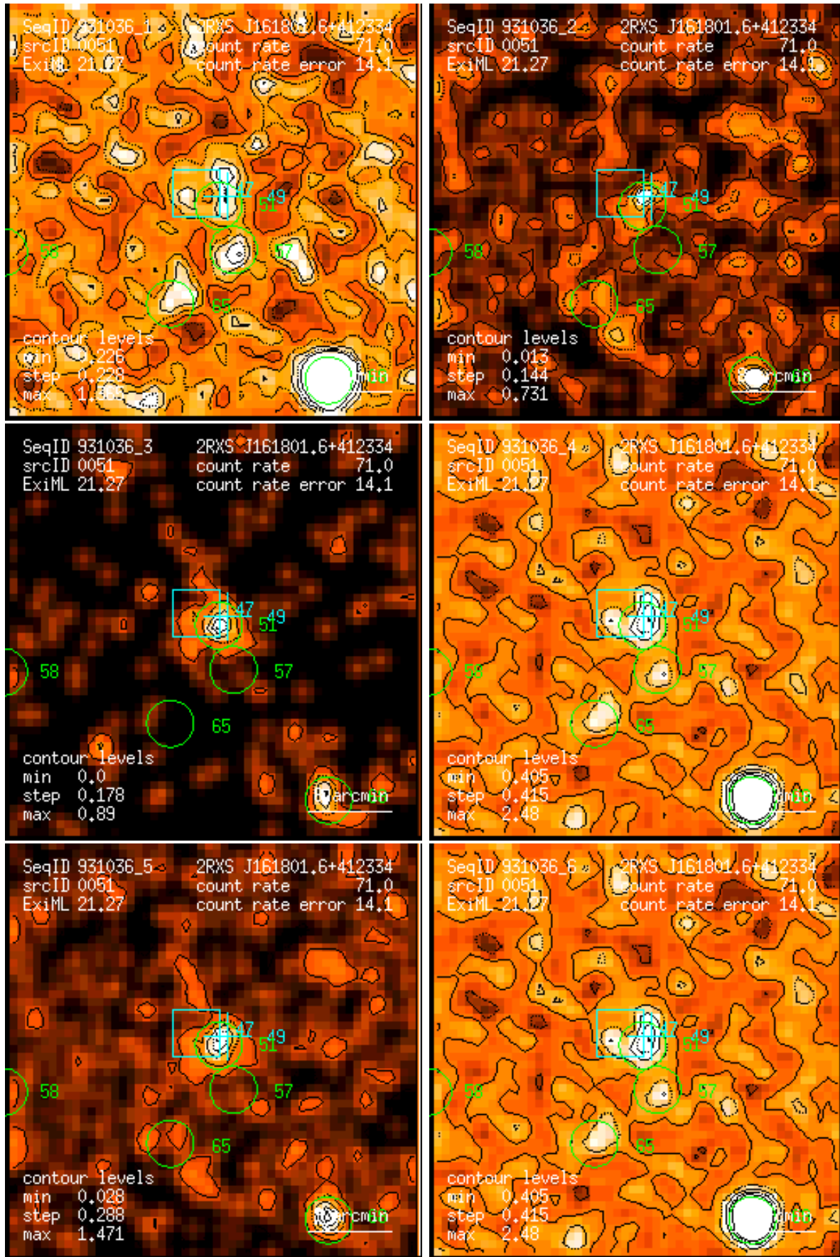
Figure 51: RASS 931036: detection 0051: band rate images, Gaussian filter: (1) PSPC channels 11 – 41, (2) 52 – 90, (3) 91 – 201, (4) 11 – 235, (5) 52 – 201, (6) 11 – 201. Broad band rates in counts/ks. Band rate contour levels in counts/ks/arcmin 2 .
