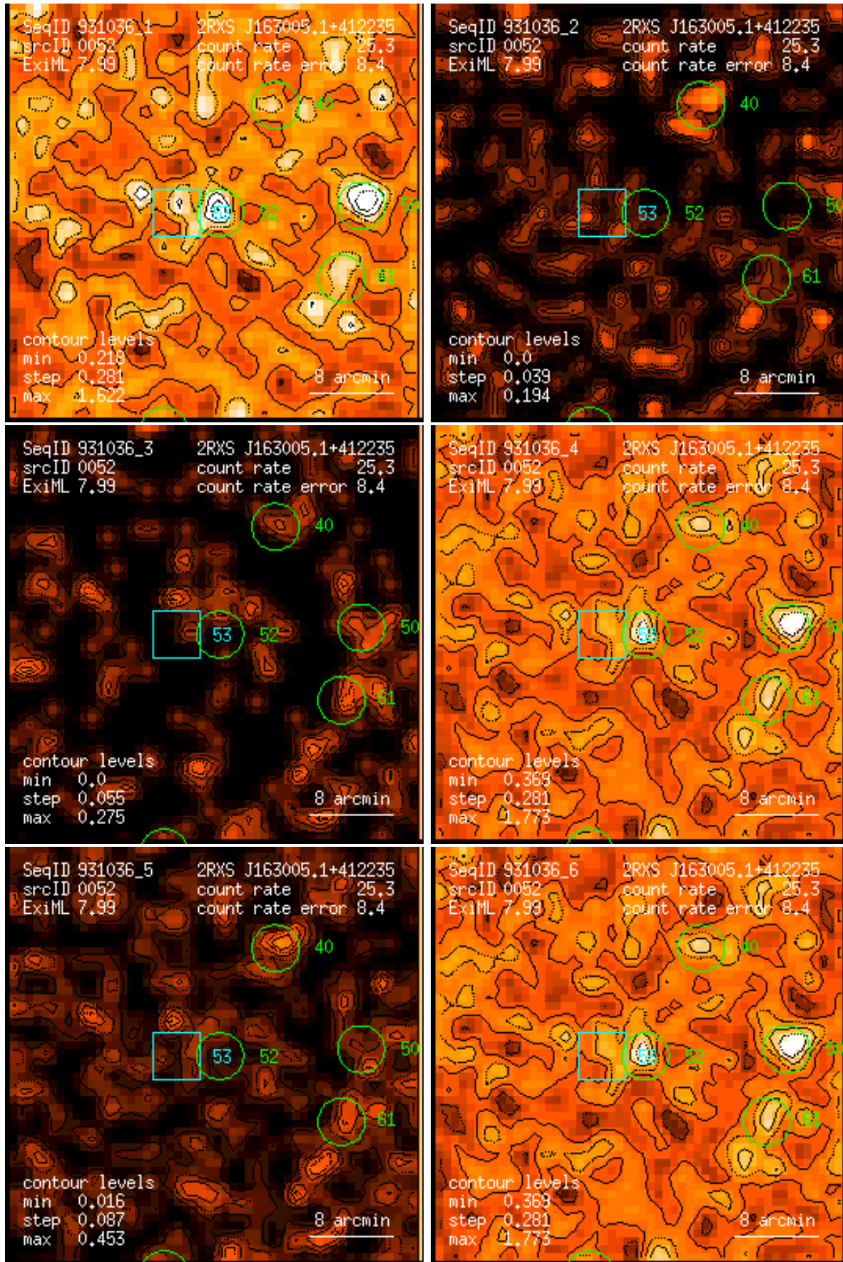
Figure 52: RASS 931036: detection 0052: band rate images, Gaussian filter: (1) PSPC channels 11 – 41, (2) 52 – 90, (3) 91 – 201, (4) 11 – 235, (5) 52 – 201, (6) 11 – 201. Broad band rates in counts/ks. Band rate contour levels in counts/ks/arcmin 2 .
