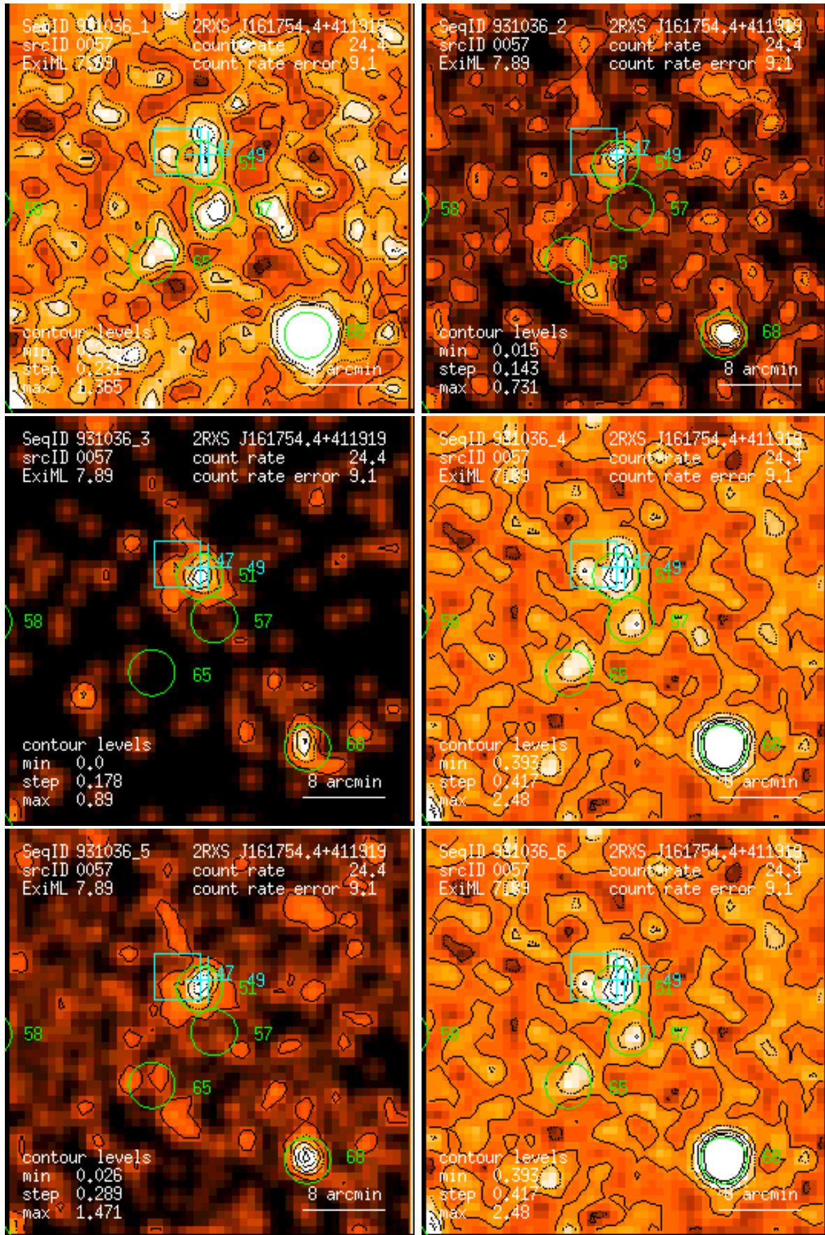
Figure 57: RASS 931036: detection 0057: band rate images, Gaussian filter: (1) PSPC channels 11 – 41, (2) 52 – 90, (3) 91 – 201, (4) 11 – 235, (5) 52 – 201, (6) 11 – 201. Broad band rates in counts/ks. Band rate contour levels in counts/ks/arcmin 2 .
