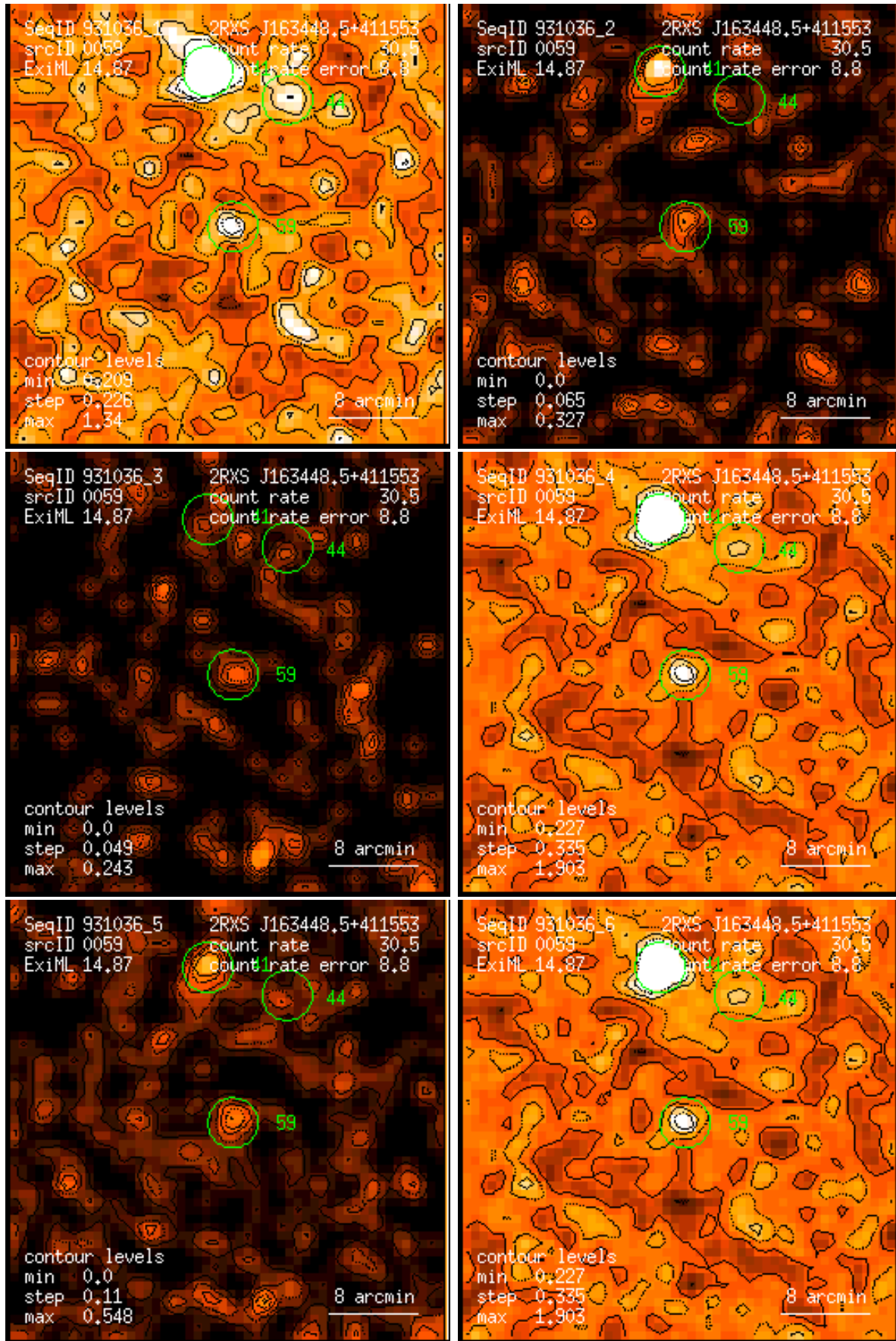
Figure 59: RASS 931036: detection 0059: band rate images, Gaussian filter: (1) PSPC channels 11 – 41, (2) 52 – 90, (3) 91 – 201, (4) 11 – 235, (5) 52 – 201, (6) 11 – 201. Broad band rates in counts/ks. Band rate contour levels in counts/ks/arcmin 2 .
